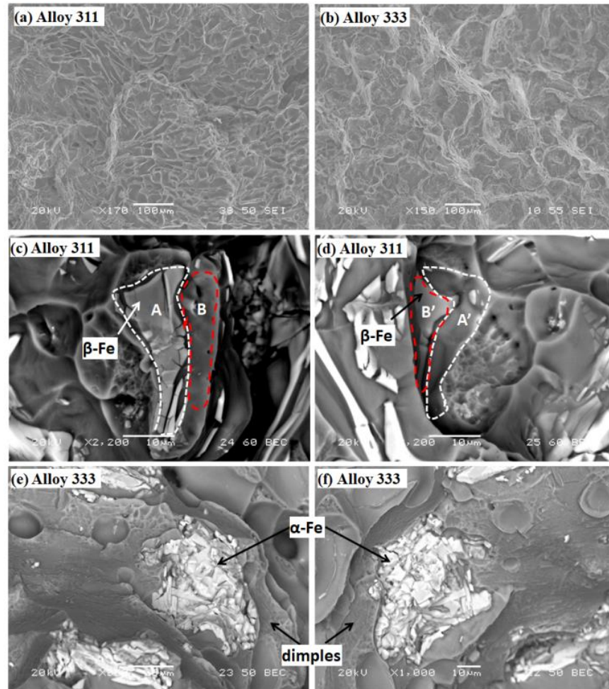
Fig. 4 Fracture surfaces of the experimental alloys (a-b) and distribution of Fe-rich intermetallics on the mating fractures (c-f)
