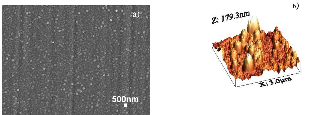
Figure 1. Bilayer surface morphology of the Al/Cr a) SEM at 5,000 X and b) AFM to 3\mu\text{m} \times 3\mu\text{m} on steel 9840.
