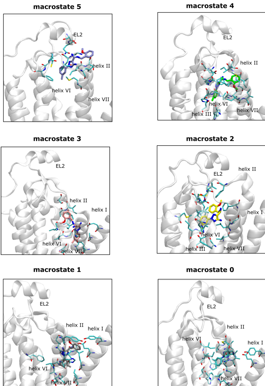
Figure S2: Representative poses adopted by Cmp-1 in each macrostate.
