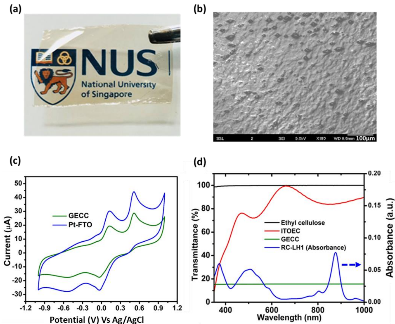
Figure 2. Properties of cell components. (a) Cast and annealed ITO-EC shows high transmittance across the visible region. (b) Scanning electron microscopy image of a GECC electrode. (c) Comparison of the catalytic activity of GECC and Pt electrodes against TMPD as a test electrolyte. (d) Transmittance of ethyl-cellulose remains high across most of the visible and near-IR when coated with ITO (selected as front electrode) but is uniformly lowered by embedded graphene nanoplatelets (selected as back electrode).
