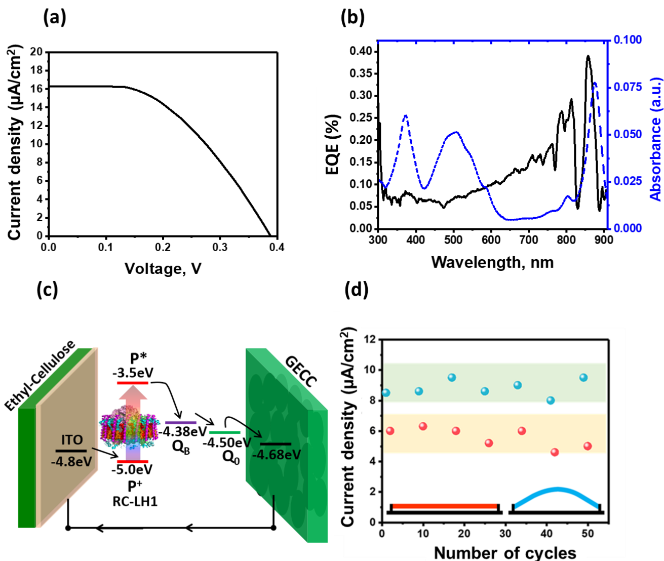
Figure 3. Output of an ITOEC/RC-LH1/Q 0 /GECC cell and effects of deformation. (a) Photocurrent-voltage response under 100 mW/cm 2 illumination. (b) Action spectrum of external quantum efficiency compared to the absorbance spectrum of the RC-LH1 pigment-protein. (c) Schematic of cell mechanism; in cells where the GECC electrode was replaced by AuEC the energy level was changed to -5.1 eV. (d) Stable photocurrent output under continuous white light illumination under bent (blue) or relaxed (red) conformations for 50 bend/relax cycles; data ranges are shaded and data points for every 8 cycles are shown. The photocurrent density was recorded after it had stabilised following each bend or relax event.
