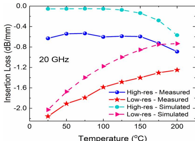
Fig. 4. Measured insertion loss (dB/mm) and simulated substrate loss (dB/mm) at 20 GHz for 160 nm SiN x on HR- and LR-Si substrates. Both simulations and experiment capture the trend of loss increasing with temperature for high-res silicon and vice-versa for low-res silicon, for reasons discussed in the text.
