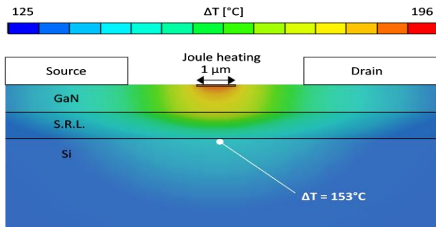
Fig. 9. Thermal simulations of a generic 4.8mm wide AlGaIn/GaN HEMT stack on Si with a nominal power density of 4 W/mm, showing the temperature rise around the channel region and the extent of temperature rise in the substrate. The Joule heating region highlighted is based on Ref.[11].
