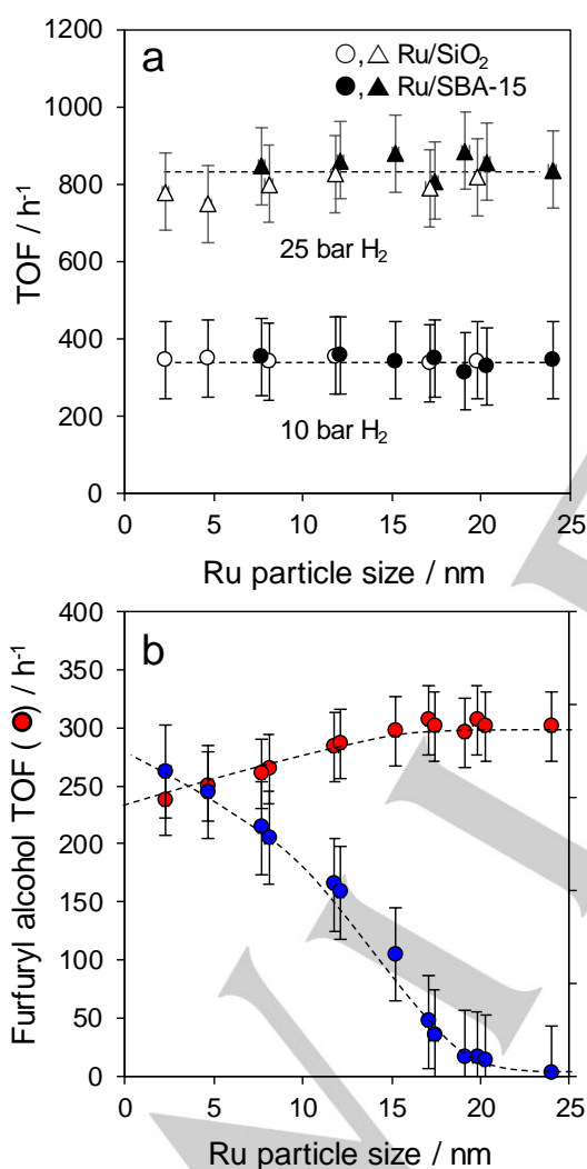
Figure 2. Turnover frequencies for (a) furfural hydrogenation at 10 and 25 bar \text{H}_2 pressure, and (b) furfuryl alcohol and furan production at 10 bar over silica supported Ru catalysts. Reaction conditions: 100 mg catalyst, 10.86 mmol furfural in 50\text{ cm}^3 toluene, 900 rpm and 100^\circ\text{C} .
