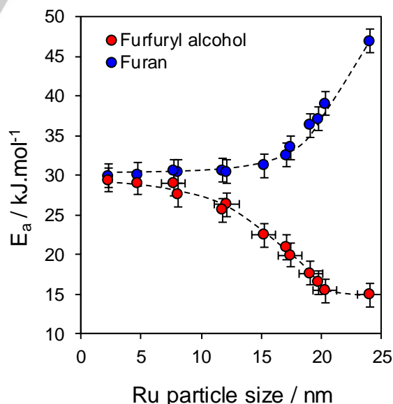
Figure 3. Influence of Ru particle size on apparent activation energy for furfural hydrogenation over silica supported Ru catalysts. Reaction conditions: 100 mg catalyst, 10.86 mmol furfural in 50\text{ cm}^3 toluene, 10 bar \text{H}_2 , 900 rpm and 100 – 165^\circ\text{C} .
