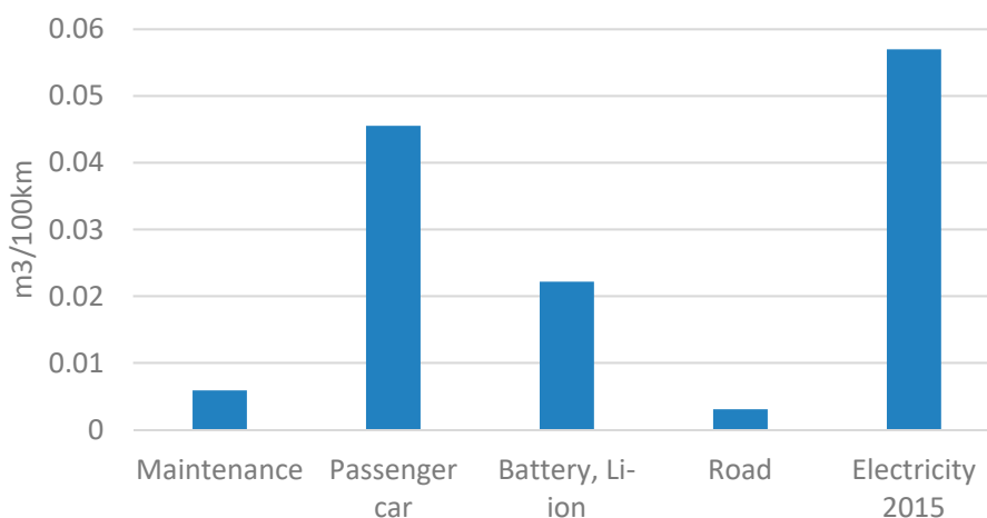
Figure 4. The water footprint of EVs in the CR in 2015.
