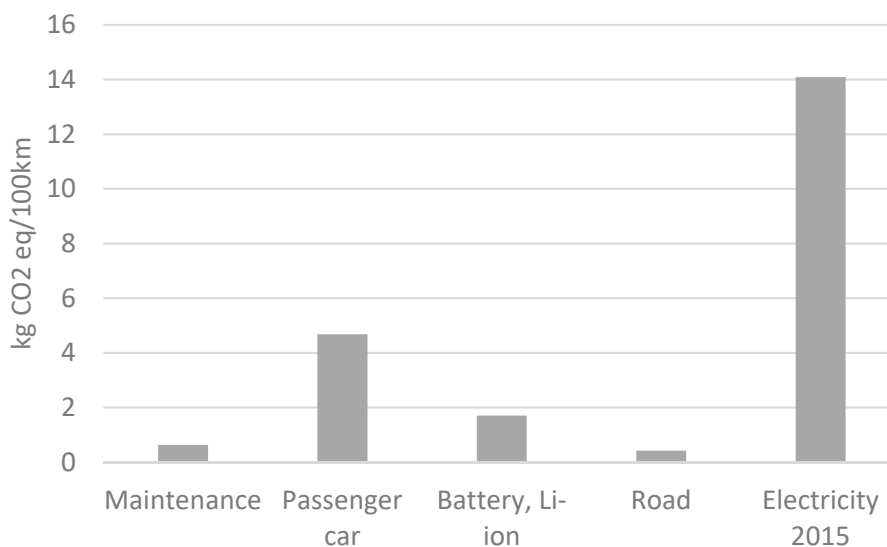
Figure 3. The carbon footprint of electric vehicles (EVs) in the Czech Republic in 2015.
