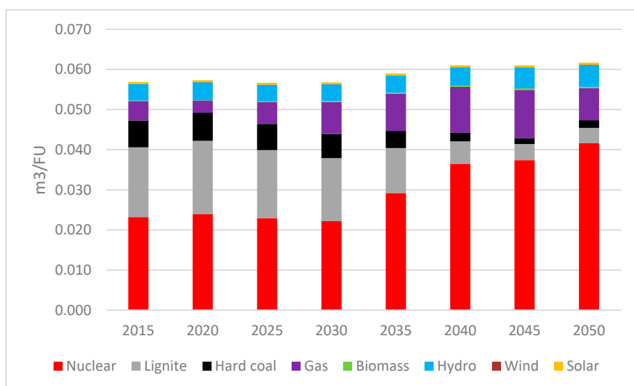
Figure 8. Results of the water footprint from electric vehicles batteries charging in the CR.
