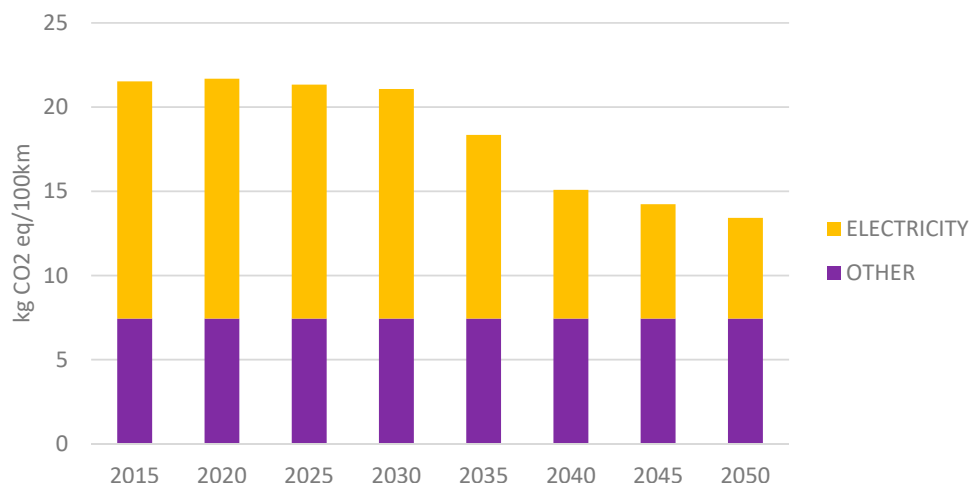
Figure 5. Results of the carbon footprint for electric vehicles in the CR (current and future).
