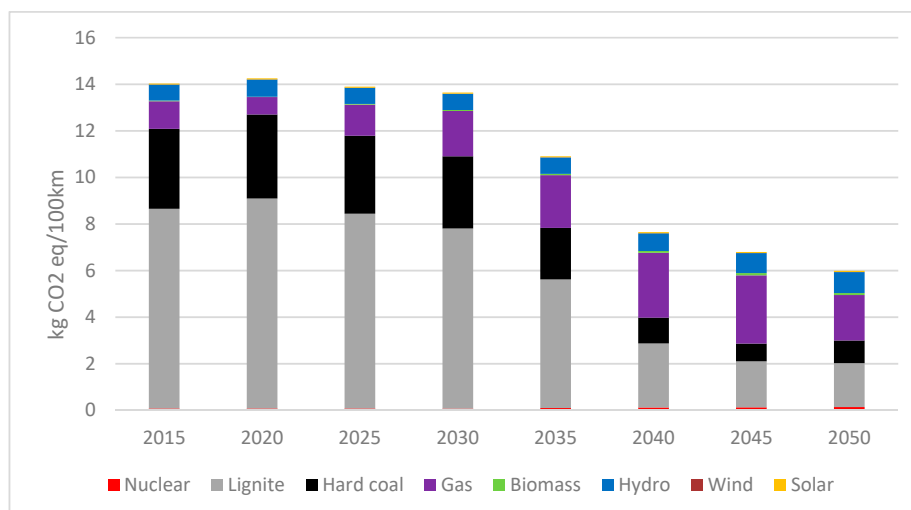
Figure 7. Results of the carbon footprint from electric vehicles batteries charging in the CR.
