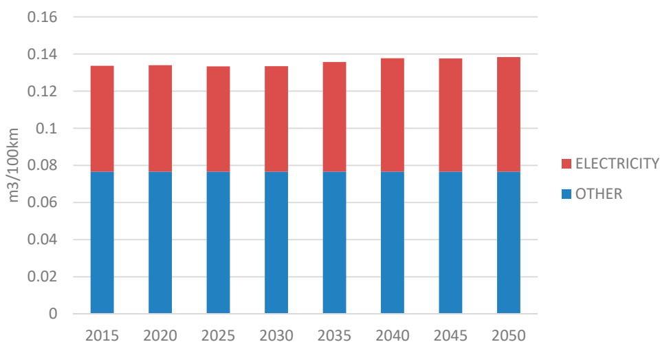
Figure 6. Results of the water footprint for electric vehicles in the CR (current and future).
