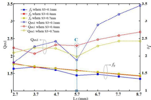
Fig. 5. External quality factor ( Q_{ex1} ) with L_4
