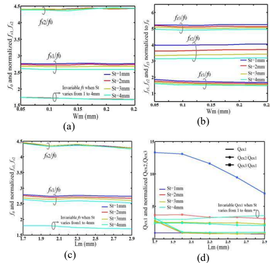
Fig. 15. The influence of W_m and L_m on the response of the APUML-ASIR Tri-band filter for variation of St: (a) f_0 and normalized f_{si} ( W_m varies); (b) Normalized f_{zi} ; (c) f_0 and normalized f_{si} , ( L_m varies); (d) Q_{ex1} and normalized Q_{ex2,3} . When one parameter varies, the others remain unchanged
