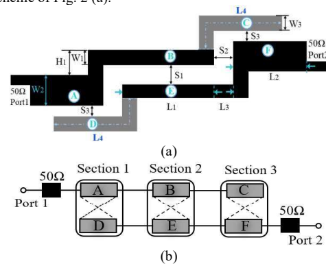
Fig. 2. A SS-ASIR coupled pair with meander coupled section. (a) The schematic diagram. (b) Equivalent circuit and coupling routing scheme for the proposed filter.
