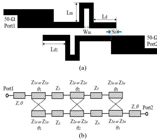
Fig. 14. The schematic diagram of the SS-ASIR coupled pair with asymmetric parallel uncoupled meander sections (a) The schematic diagram. (b) Even-mode or odd-mode equivalent circuit
