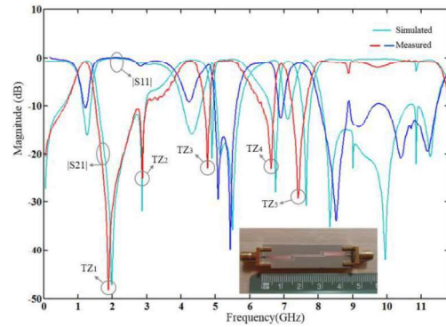
Fig. 13. Simulated and measured results, and photograph of a modified quint-wideband type SSMCL-ASIR
