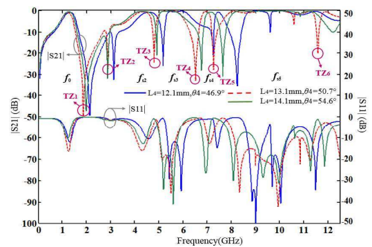
Fig. 11. Variation of S_{11} and S_{21} versus different values of L_4
