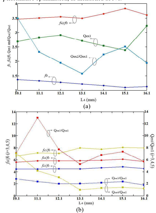
Fig. 12. The effect of L_4 on quint-wideband type SSMCL-ASIR (a) f_0 , Q_{ex1} , f_{s2}/f_0 and Q_{ex2}/Q_{ex1} versus against L_4 , (b) f_{s1}/f_0 and Q_{ex3}/Q_{ex1} ( i = 3, 4, 5 ) versus against L_4
