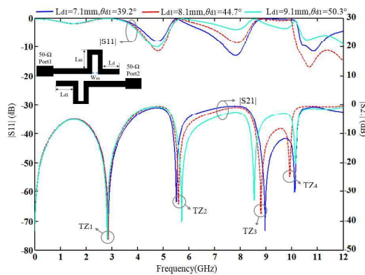
Fig. 17. The analysis of the APUML structure
