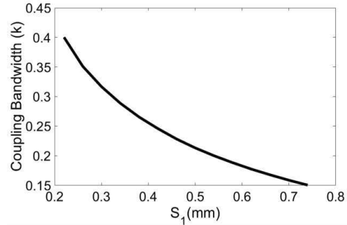
Fig. 6. Coupling Bandwidth (K) with the gap size ( S_1 )
