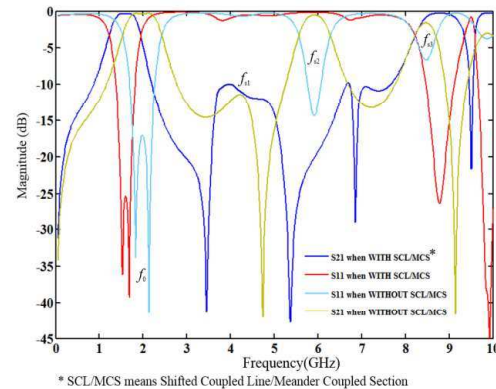
Fig. 3. Frequency response comparison with and without SCL/MCS.
