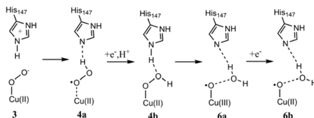
Scheme 6. Proposed mechanisms for \text{O}_2 activation by LPMO from Ref. 6.
