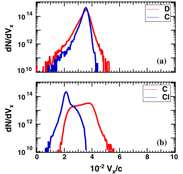
FIG. 7. Velocity spectrum of the expanding ions in (a) CD and (b) \text{CCl}_2 targets taken at \Delta x = 3 \mu\text{m} in the upstream region at t = 4.0 \text{ ps} .
