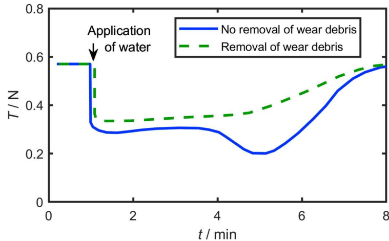
Figure 1: Results from Amsler twin disc experiments [2] showing that wear debris (iron oxides) are necessary to significantly reduce the adhesion T/N (where T and N are the tangential and normal forces, respectively).
