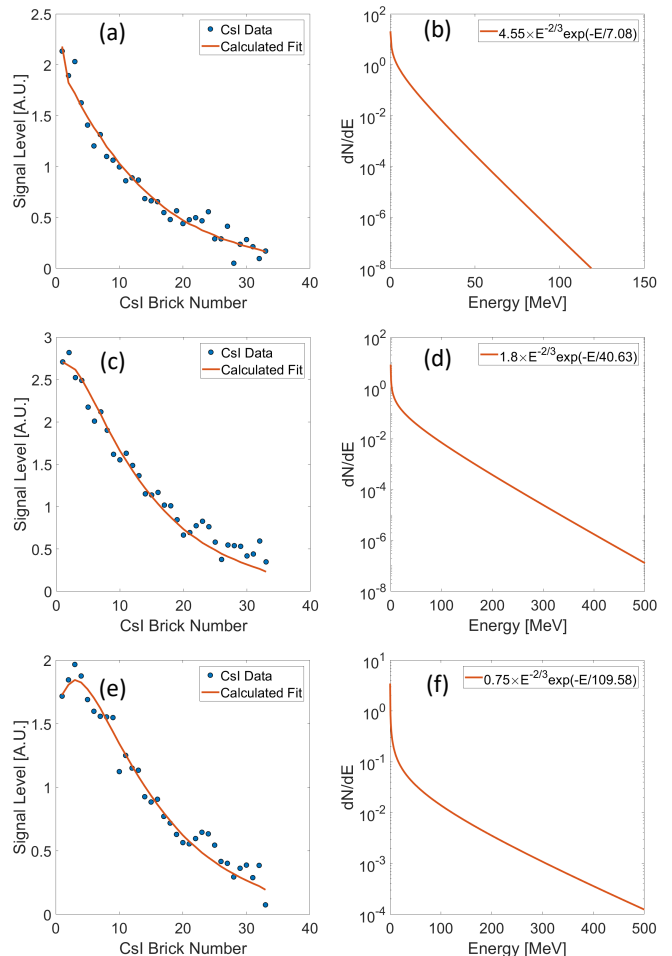
FIG. 5. Data and calculated fit plotted with corresponding spectra. The data obtained from the CsI detector is marked with the blue dots and the calculated fit is plotted as the solid line among the dots. (a) + (b) Example of a low critical energy fit and spectrum of E_{crit} = 7.08 MeV. (c) + (d) Example of a moderate critical energy fit and spectrum with E_{crit} = 40.63 MeV. (e) + (f) Example of a high critical energy fit and spectrum with E_{crit} = 109.58 MeV.
