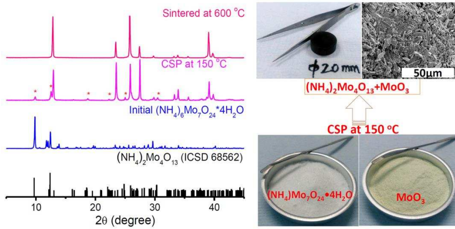
Fig. 4 XRD patterns of the starting (\text{NH}_4)_6\text{Mo}_7\text{O}_{24}\cdot 4\text{H}_2\text{O} powder, cold sintered \text{MoO}_3 ceramic with (\text{NH}_4)_6\text{Mo}_7\text{O}_{24}\cdot 4\text{H}_2\text{O} (150 °C for 0.5 h) and a sample annealed at 600 °C, and optical and SEM images of the starting powders and cold sintered \text{MoO}_3 ceramics.
