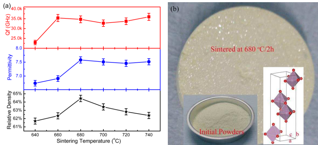
Fig. 1 a) Relative \rho , \epsilon_r and Qf value of MoO 3 ceramics prepared via conventional sintering as a function of sintering temperature (640 ~ 740 °C). b) Optical images of starting powder and MoO 3 ceramic sintered at 680 °C / 2 h with its crystal structure inset.
