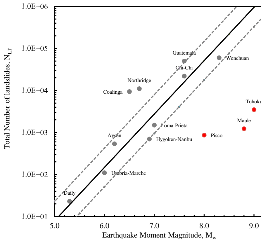
Figure 9. Dependence of Total number of landslide N_{LT} and earthquake moment magnitude M_w to shallow crustal (grey) and megathrust (red) earthquakes. Solid line is the correlation from the relationship proposed by Malamud et al. (2004b) with the grey dashed lines providing the corresponding error bounds. Data for the 13 earthquakes are given in Table 2 of supplementary material (S1).
