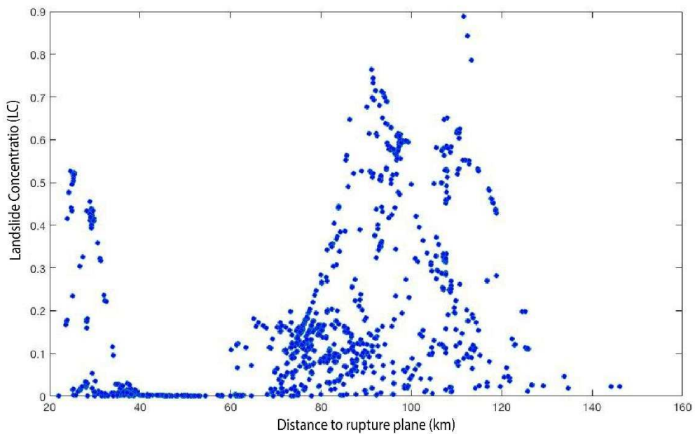
Figure 8. a) N° landslides vs distance to rupture plane. b) LC vs Distance to rupture plane
