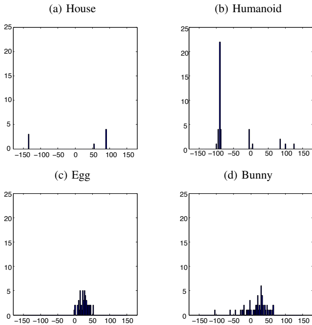
Fig. 17. The histograms of the fold angles. The x-axis is fold angles. The y-axis is frequency. The width is 2.5°.
