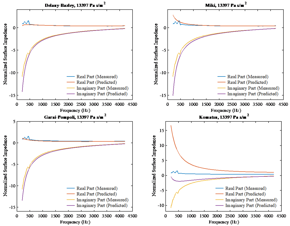
Figure C4. Measured and predicted impedance for the sample with airflow resistivity of 13397 Pa·s/m 2 .
