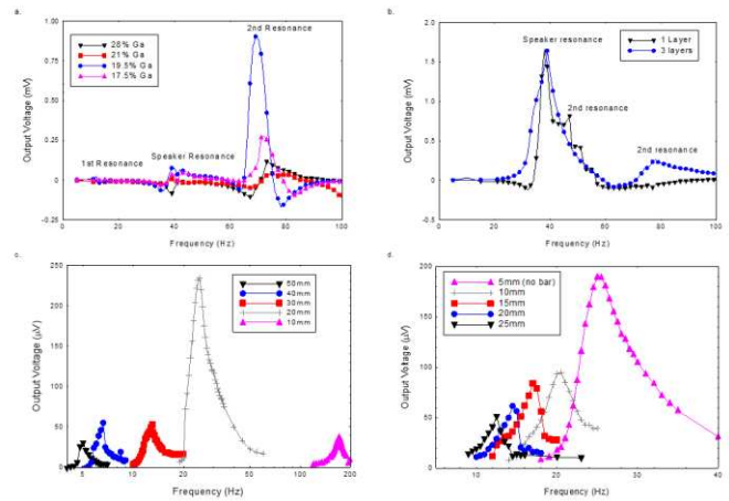
Fig. 4. Voltage as a function of frequency for a. FeGa cantilevers, b. Metglas cantilevers (layer thickness 18 \mu m), c. Metglas cantilevers (layer thickness 60 \mu m) and d. Metglas T-bar cantilevers
