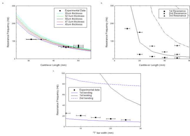
Fig. 5. Comparison between the modelling data and the resonance frequency for different dimension cantilevers a. FeGa, b. Metglas (layer thickness 60μm) and c. “T” bar cantilevers
