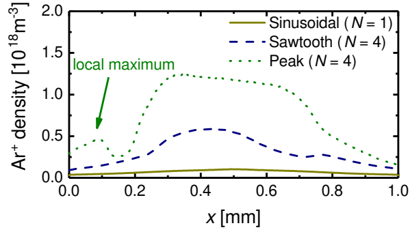
Figure 2. Time-averaged \text{Ar}^+ density profile for sinusoidal, sawtooth-up and peak waveforms.
