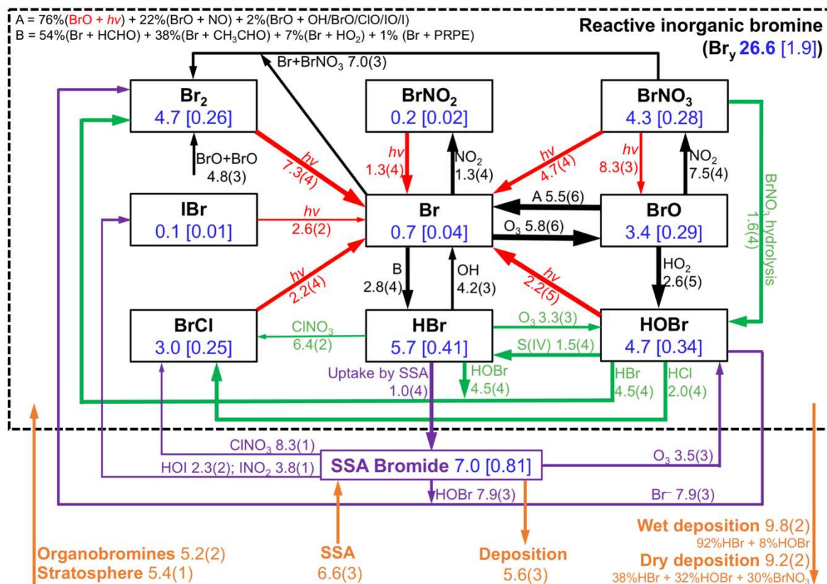
5 Figure 3. Global annual mean tropospheric budget and cycling of reactive inorganic bromine ( \text{Br}_y ) and sea salt aerosol (SSA) bromide. Results are from our GEOS-Chem simulation for 2012 including SSA debromination. \text{Br}_y is defined as the ensemble of species inside the dashed box. Rates are in \text{Gg Br a}^{-1} , masses in the boxes are in \text{Gg Br} , and numbers in brackets are mean mixing ratios (ppt). Read 2.8(4) as 2.8 \times 10^4 \text{ Gg Br a}^{-1} . Arrows in black are for gaseous reactions, red for photolysis, purple for heterogeneous reactions in SSA, and green for other heterogeneous reactions taking place in cloud and sulfate aerosol. Sources and sinks of total inorganic bromine ( \text{Br}_y + \text{SSA bromide} ) are in orange. Arrow thickness scales with its corresponding rate.
