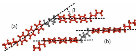
Figure 4 – (a) Estimated N_{tb} conformation with \beta = 32^\circ ; this produces \alpha = 67^\circ when tilted 30^\circ to the helical axis. Shown at a different angle to Figure 3a. (b) Parallel conformation representing torsional maximum.
