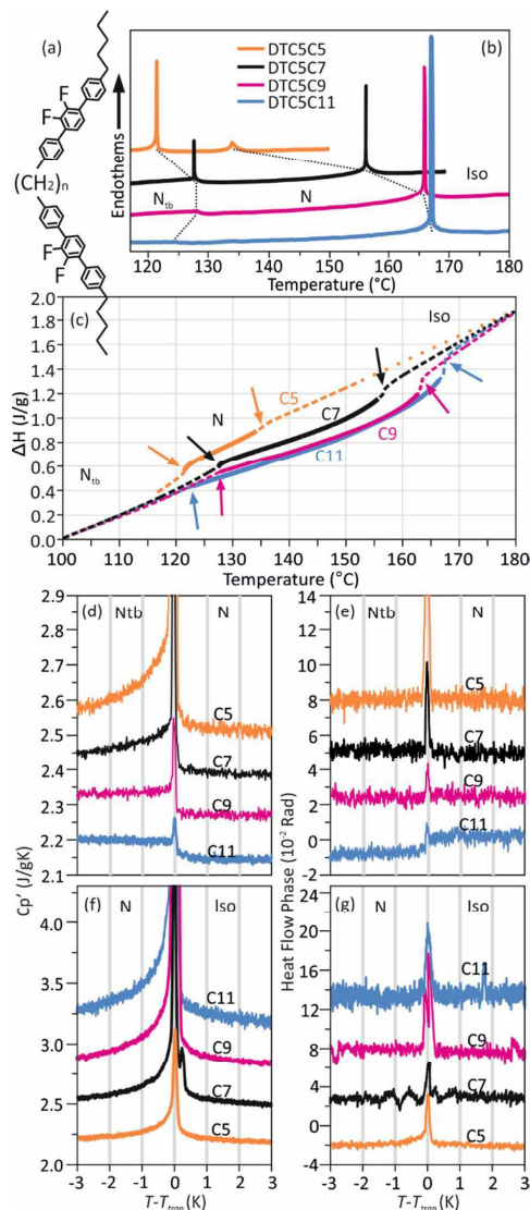
Figure 1 – (a) Chemical structure of DTC5C n compounds. (b) Standard DSC heating thermograms (3 K/min) of DTC5C n compounds showing N tb -N and N-Iso transitions. Each curve in panels b-f is labelled by spacer length n . (c) Temperature dependence of cumulative enthalpy relative to H_{100^\circ\text{C}} . Bold solid = N phase; arrows indicate transitions. (d) MDSC C_p' curves \pm 3\text{K} of T_{N_{tb}-N} . (e) Heat flow phase \phi vs T corresponding to (d). (f) MDSC C_p' curves \pm 3\text{K} of T_{N-Iso} . (g) Heat flow phase \phi vs T corresponding to (f). In panels d-f baselines have been shifted for display.
