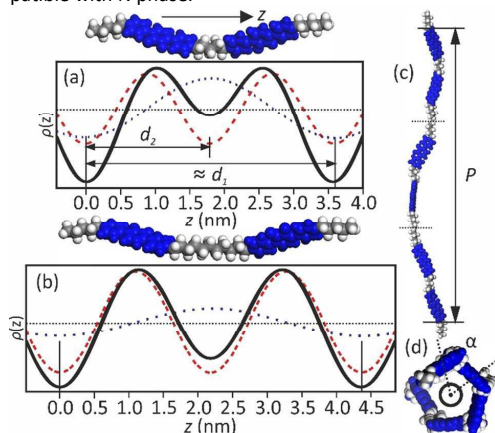
Figure 3 – a,b) Simplified 1D electron density profiles of N_{tb} phase in (a) DTC5C5 and (b) DTC5C11, reconstructed from SAXS intensities along the meridian. Blue/red dashes show separate contributions of q_1/q_2 to \rho(z) (solid black). \psi = \pi for both contributions. The horizontal dotted line is the average electron density. Model molecular conformations matching the density profiles are also shown to aid interpretation. The overlaying molecules have been altered in size to coincide with the d_1=2d_2 lamellar approximation. (c) N_{tb} helix with curved molecular trajectory shown on the example of DTC5C5, P = pitch length. (d) View of (c) along P .
