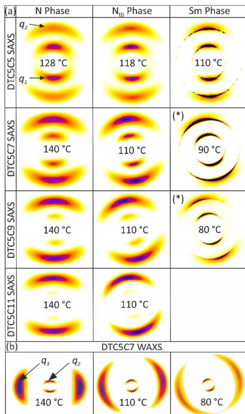
Figure 2 – (a) SAXS and (b) WAXS patterns of magnetically aligned DTC5C n compounds in the three LC phases; magnetic field direction is always vertical, B = 2.5T . *Phases only observed on cooling. The WAXS patterns in (b) are of DTC5C7, but appear similar in all compounds.
