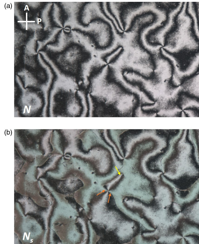
FIG. 4. Polarization microscopy images in (a) N ( 135^\circ\text{C} ) and (b) N_S ( 125^\circ\text{C} ) phases in a homeotropic cell (thickness 18 \mu\text{m} ). The appearance of two additional defect lines around \pm 1 defects and one around \pm 1/2 defects in the N_S phase indicates that the symmetry of this phase is lower than that of the N phase. The polarizer and analyzer are oriented as shown in (a). The width of the images is 545 \mu\text{m} . The yellow and orange arrows point at additional lines around one \pm 1/2 and one \pm 1 defect, respectively.
