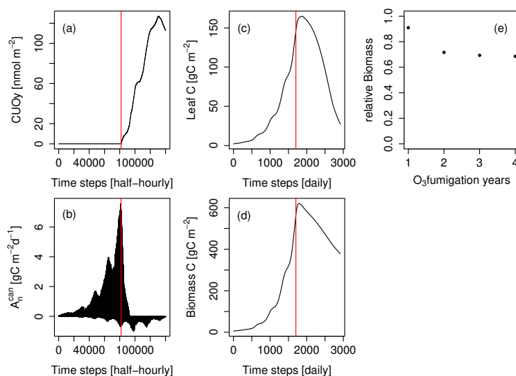
Figure 2. Cumulative ozone uptake above a threshold of 0.8 \text{ nmol m}^{-2} (\text{leaf area}) \text{ s}^{-1} ( CUOY ), canopy integrated net photosynthesis ( A_n^{can} ), leaf carbon content ( Leaf C ), total carbon in biomass ( Biomass C ) and relative Biomass ( RB ) of Pinus halepensis at the Ebro Delta fumigated with the NF+ ozone treatment. Simulations are conducted with the L12_{PS} model version. Panels a-d display the entire simulation period. The red line indicates the onset of O_3 fumigation (NF+) in the 5th of 8 simulation years. The relative biomass compared to a control simulation with zero O_3 concentration (panel e) is displayed for the O_3 fumigation years.
