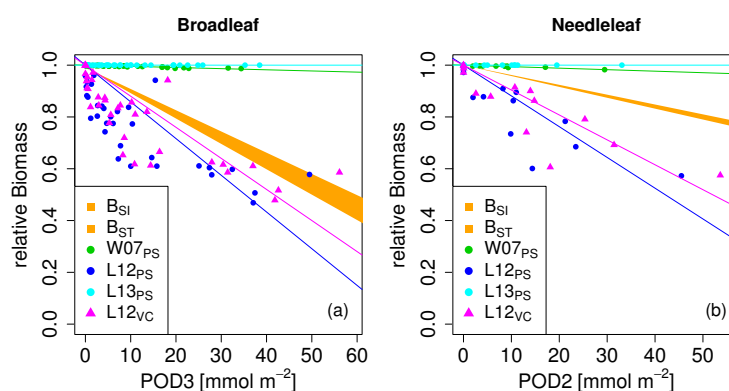
Figure 1. Biomass dose-response relationships for simulations based on published damage relationships, separate for a) broadleaved species, and b) needle-leaved species. The dose-response relationships by B ker et al. (2015), B_{SI} and B_{ST} , define the target area (orange). The displayed dose-response relationships are simulated by model versions which base damage calculations either on net photosynthesis W07_{PS} (Wittig et al., 2007), L12_{PS} (Lombardozzi et al., 2012a), and L13_{PS} (Lombardozzi et al., 2013), or on V_{cmax} L12_{VC} (Lombardozzi et al., 2012a) (see Tab. 1 for more details). See Tab. A.3 and A.4 for slopes, intercepts, R^2 and p-values of the displayed regression lines. Damage calculation in the simulations bases on CUOY (see Tab. 1) and not on POD2 or POD3 (see Sec. 2.4 for more details).
