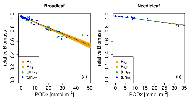
Figure 3. Biomass dose-response relationships for simulations based on tuned damage functions (see Tab. 1 for abbreviations), separate for a) broadleaved species, and b) needle-leaved species. The dose-response relationships by Büker et al. (2015), B_{SI} and B_{ST} , define the target area (orange). See Tab. A.5 and A.6 for slopes, intercepts, R^2 and p-values of the displayed regression lines. Damage calculation in the simulations base on CUO1 (see Tab. 1) and not on POD2 or POD3 (see Sec. 2.4 for more details).
