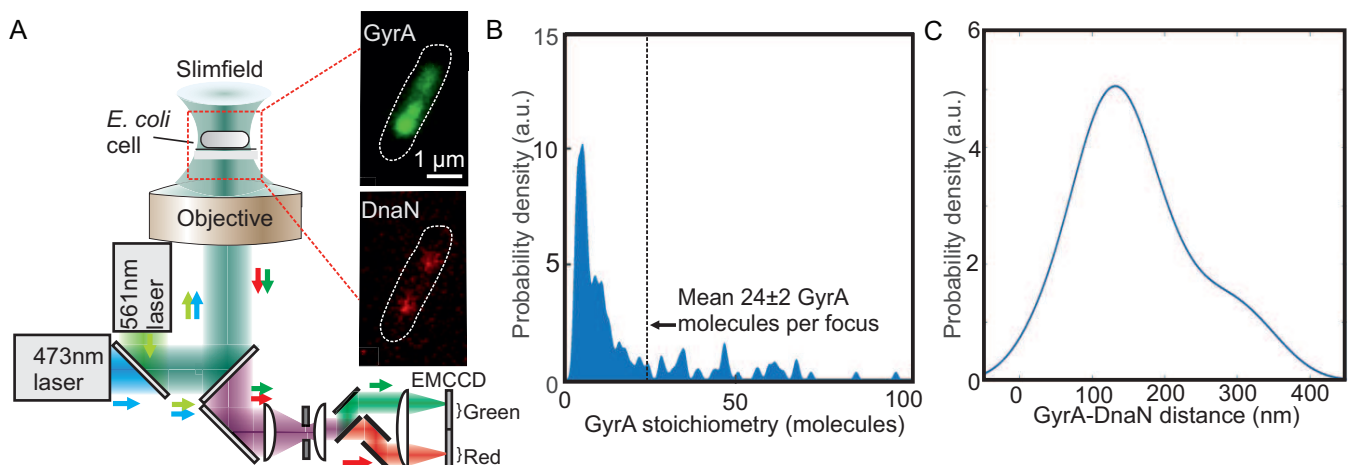
Figure 3. Gyrase foci of a few tens of molecules. (A) Dual-color Slimfield enables single-molecule tracking in two separate color channels with millisecond sampling, for the strain Gyrase-mYPet:DnaN-mCherry, cell outline indicated (white dash). (B) Stoichiometry distribution rendered as a kernel density estimate (42) for all detected Gyrase-mYPet foci, mean ( \pm SEM) indicated for all Gyrase, kernel width 0.7 molecules. (C) Distribution of displacements between foci centers for colocalized DnaN and Gyrase rendered as a kernel density estimate, kernel width 40 nm. Data acquired from 72 foci using N = 35 cells.
