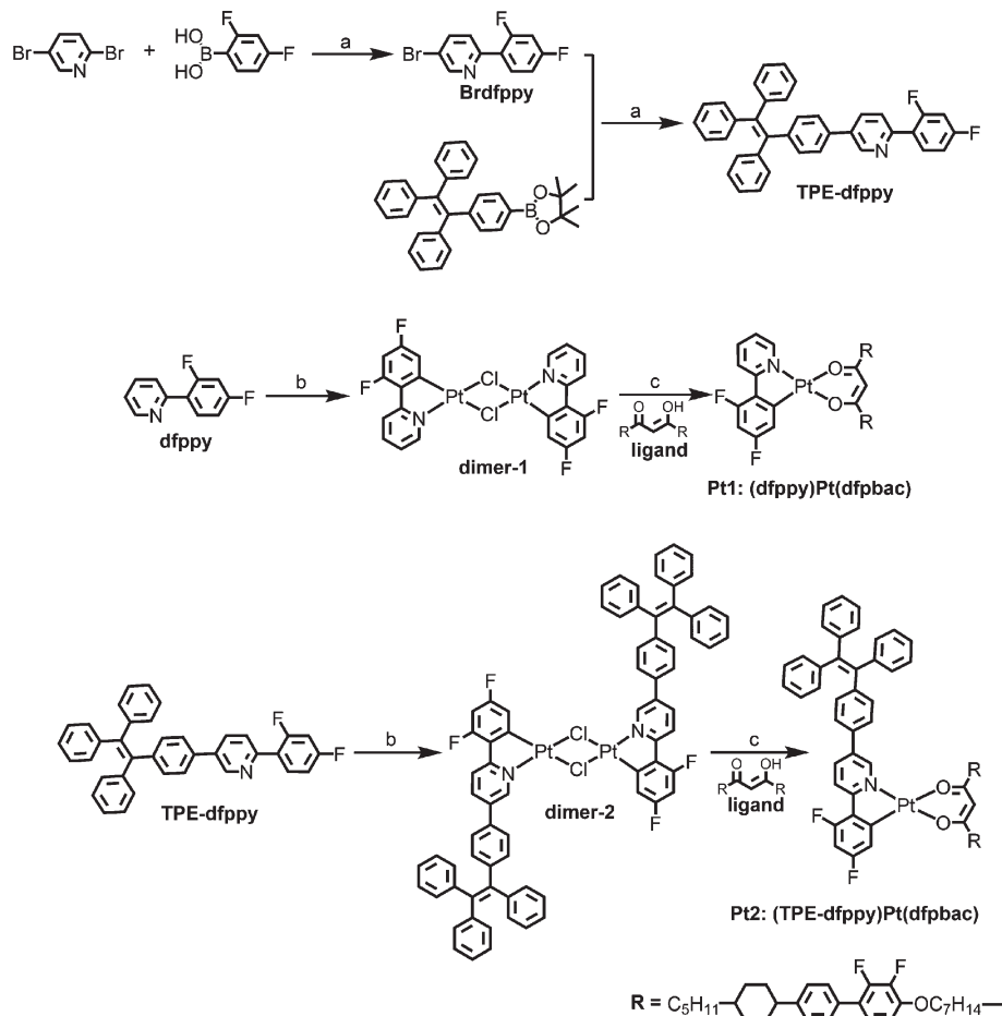
Scheme 1 Synthetic route of platinum complexes. (a) K 2 CO 3 , [Pd(PPh 3 ) 4 ], THF, reflux, overnight; (b) K 2 [PtCl 4 ], 2-ethoxyethanol, H 2 O, 80 °C, 24 h; (c) acac derivative, Na 2 CO 3 , 2-ethoxyethanol, 100 °C, overnight.
