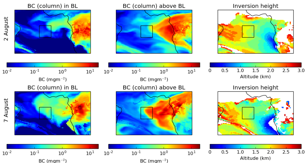
Figure 2. Black carbon (BC) column mass above and below the inversion (or above and below 1300 m altitude, if a clear inversion could not be diagnosed) in the global model on 2 and 7 August, and the inversion height on these days. Where 1300 m altitude is used because there is no inversion, or where the inversion height is over 2800 m above the surface, the right-hand plots are white. The marked square is the domain of the regional model.
