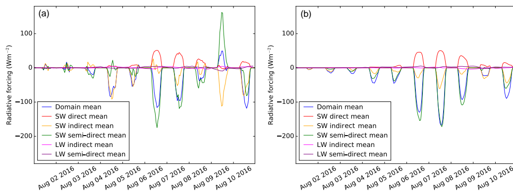
Figure 16. Decomposition of the radiative effects of biomass burning smoke in the regional model domain in the global model (a) and the regional model (b) into the direct, indirect and semi-direct components in the short- and longwave bands according to the recommendations by (Ghan et al., 2012).
