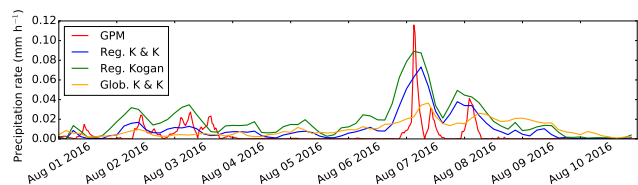
Figure 11. Domain mean precipitation rate in the regional and global models, in \text{mm h}^{-1} , compared with the GPM dataset (Huffman et al., 2014). The effect of the biomass burning aerosol on rain is shown later, in Fig. 14.
