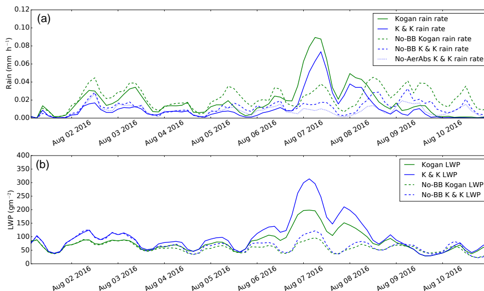
Figure 14. Domain mean precipitation rates (a) and liquid water path (b) in the regional model with and without biomass burning emissions, with the alternative parameterisations of autoconversion and accretion from (Kogan, 2013) and from (Khairoutdinov and Kogan, 2000) (labelled K & K).
