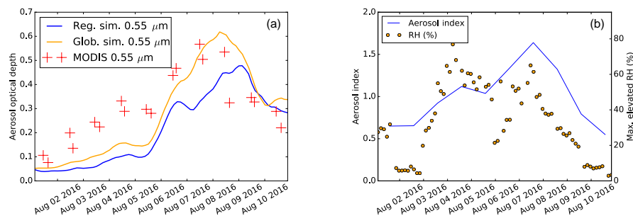
Figure 8. (a) Aerosol optical depth, averaged over the regional domain. We did not attempt to correct sampling biases: retrievals in the MODIS aerosol optical depth domain average are not given greater weight when they are further away from other retrievals, so cloudy areas where there are few AOD retrievals do not contribute as much to the domain average as areas where the skies are clear and there are many retrievals. As large areas of the regional domain have no retrievals because they are cloudy, at the edge of swaths, or in the glint regions, this bias is probably significant, but it is likely to explain some of the scatter, rather than the trend, shown in the figure. (b) OMPS aerosol index in a 7 \times 7^\circ latitude–longitude box centred on Ascension Island and maximum relative humidity above the boundary layer, measured by the ARM site sondes (Holdridge et al., 2016b).
