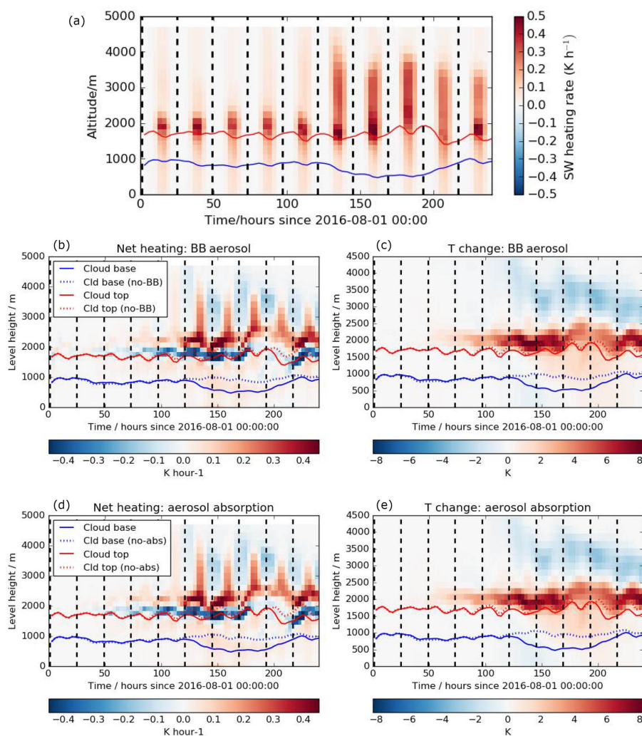
Figure 12. Regional average shortwave heating rate (a) and changes to heating rate and temperatures when biomass burning aerosol is introduced to the regional model (b, c) and when aerosol absorption of radiation is switched on (d, e). The domain mean cloud top and cloud base heights in the simulations used are marked on the plots. On each day, midnight local time is indicated by a black dotted line.
