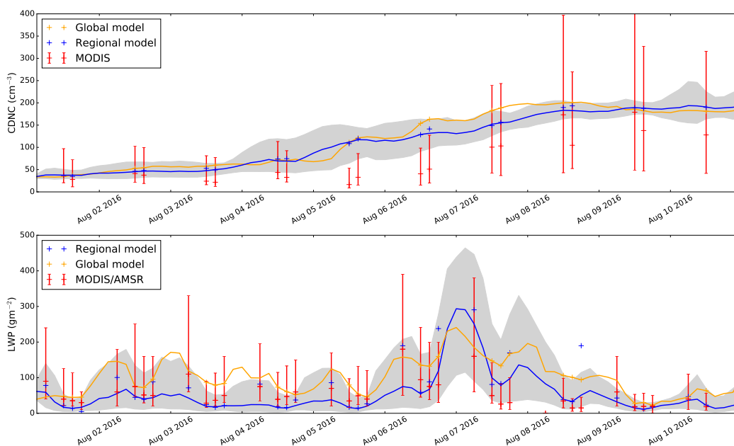
Figure 9. Time series of cloud droplet number concentration at the cloud top and in-cloud liquid water path in the model (a median within approximately 800 km of the centre of the domain) compared to corresponding AMSR and MODIS observations across the same area at matched times. The MODIS data were regridded to the resolution of the regional model. Cloudy grid boxes are defined as those with LWP above 10 \text{ g m}^{-2} . The interquartile ranges in the satellite data are shown as error bars, and the range (inner half of the distribution) in the regional model as a grey band. Where the blue crosses deviate from the overall domain median indicated by the blue lines, the regional model data were regridded to the AMSR resolution and averaged only inside the AMSR swaths, or calculated only inside the MODIS swaths. Thus the blue and red crosses are directly comparable. No correction for swaths was made in the lower resolution global model data; hence, the orange crosses lie on the orange lines and the blue and red crosses are only approximately comparable with the orange crosses. The effects of smoke aerosol on these quantities are presented and discussed later, in Fig. 15.
