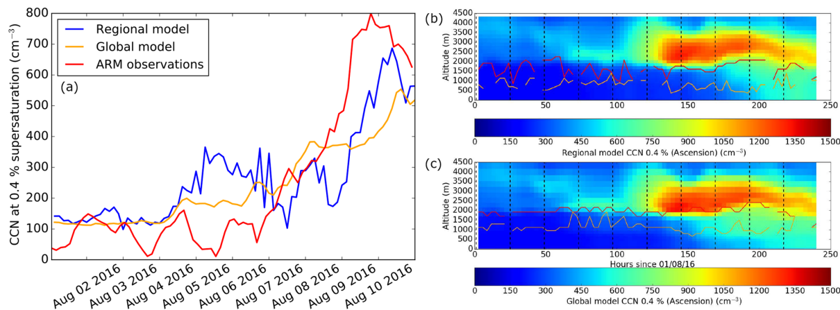
Figure 6. (a) CCN at 0.4 % at Ascension at the surface measured with the ARM CCN counter (Holdridge et al., 2016a) and compared to our simulations, and (b) the vertical profiles of CCN in the global and regional models, averaged over the domain. The cloud top and cloud base heights at Ascension Island itself are marked in red and orange respectively. The black dotted lines indicate midnight, local time.
