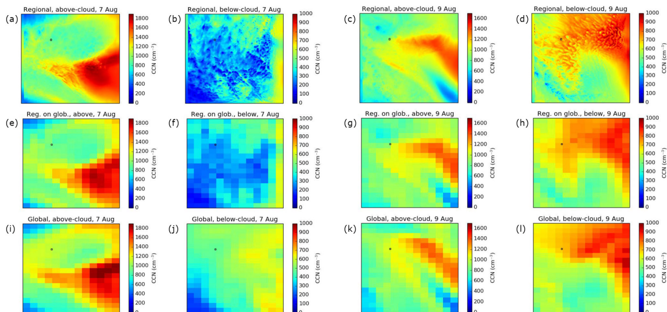
Figure 7. Snapshots of CCN at 0.4 % supersaturation across the regional model domain, in the regional and global models. The left six plots show the time of the AQUA overpass on 7 August, also shown for the regional model in Fig. 10. The right six plots show 00:01 UTC on 9 August, when the aerosol plume covers different parts of the domain. Within each group, the top plots are for the regional model and the bottom for the global model, left between the domain mean cloud top height and 3500 m altitude, and right, below the domain mean cloud top height. Note that clouds extend slightly above the domain mean cloud top height in the western half of the domain. The centre plots are for the regional model, regridded to the same resolution as the global model. The small black square represents Ascension Island.
