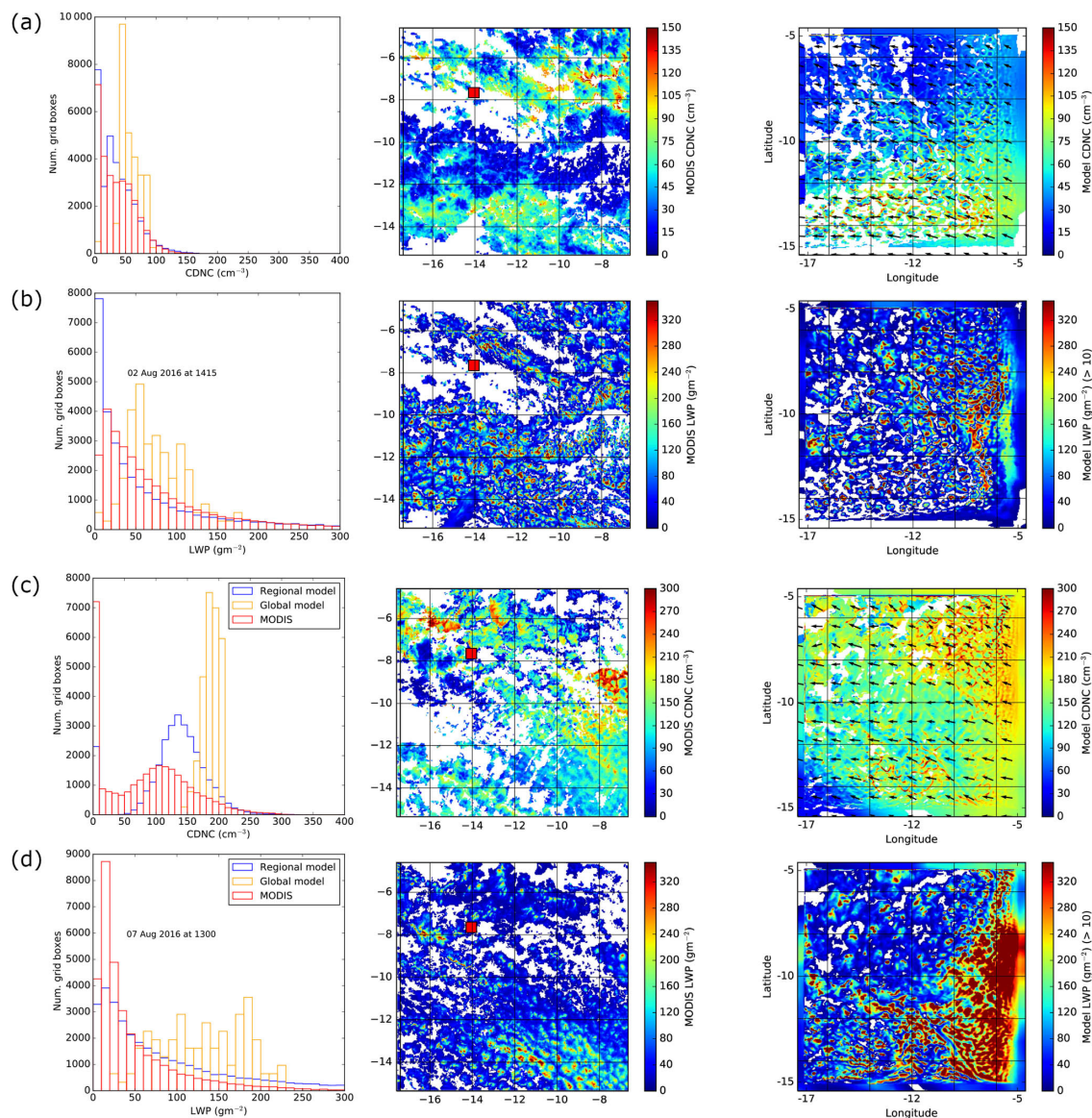
Figure 10. CDNC and LWP from MODIS AQUA and the model on 2 August ( a , b ) and 7 August ( c , d ). Wind vectors at 1260 m altitude are shown on the CDNC plot. On 7 August, the lower half of the MODIS CDNC retrieval is compromised by high cloud or aerosol, and the white areas in the CDNC plot that are not present in the LWP plot have been screened out because the cloud top temperature indicates cloud top heights are above the boundary layer.
