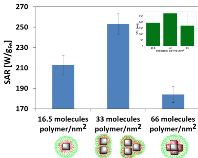
Figure 5. SAR values for soft colloidal nanoclusters after 1 year aging time, formed at ratios of 16.5, 33, and 66 molecules PScMA/nm 2 of particle surface ( f = 302 kHz, H = 23.8 kA/m). A higher SAR value was recorded for dimers and trimers compared to individual IONCs and clusters with n \geq 4 . Clustering the IONCs in centrosymmetric bead-like structures decreased their heating performance. Each experimental data point was calculated as the mean value of at least three independent measurements, with error bars indicating the mean deviation. Inset: SAR values obtained from kinetic Monte Carlo modeling of the structures as described in the text, reproducing the observed experimental trend within the error bar. Interparticle spacing for the simulation has been set to 1 nm gap as measured on the TEM images.
