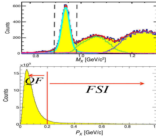
Fig. 8 Top panel Missing-mass distribution of the reaction \gamma d \rightarrow K^+ \Lambda X fitted with contributions from \gamma d \rightarrow K^+ \Sigma^0 X (green), \gamma d \rightarrow K^+ \Sigma^+ X (purple), and accidental events (magenta) from simulated data. The vertical dotted lines indicate the cuts that select the events of interest and the fits are used to perform background subtraction. Bottom panel Missing momentum of the reaction \gamma d \rightarrow K^+ \Lambda X indicating the cut applied to select FSI (Colour figure online)
