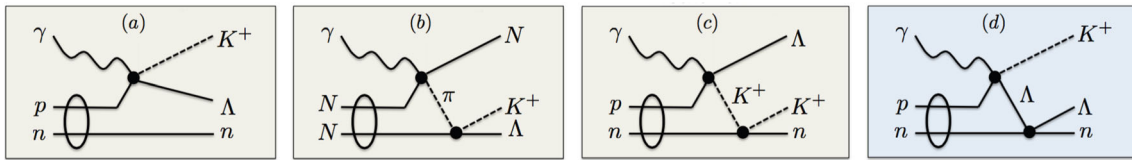
Fig. 6 Four main mechanisms that contribute to the reaction \gamma d \rightarrow K^+ \Lambda n according to theoretical models [16,17]: a quasi-free \Lambda photoproduction on the proton; b pion mediated production; c K^+ rescattering on spectator neutron; d \Lambda rescattering on spectator neutron (Colour figure online)
