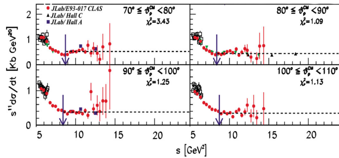
Fig. 4 Published results on the invariant cross section of the \gamma d \rightarrow pn reaction for four angles in the proton c.m. [7]. The cross section data are scaled by s^{11} to test predictions of the dimensional scaling laws. Results from CLAS are shown with the red points. The vertical arrows indicate the s value corresponding to p_{\perp} = 1.1 GeV/c and the dashed lines are fits to the data above p_{\perp} = 1.1 GeV/c (Colour figure online)
