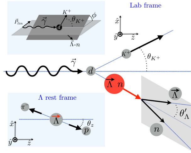
Fig. 7 Reaction plane definition for \gamma d \rightarrow K^+ \Lambda n . The upper left panel defines the kaon azimuthal angle \phi , in which \Sigma produces a modulation (see Eq. 1). The lower left panel shows the definition of \theta_z (and correspondingly \theta_x ) in which the double polarisation observables produce modulations. The kaon polar angle and the hyperon angle \theta'_\Lambda , which polarisation observables are predicted to be sensitive to are defined in the main figure
