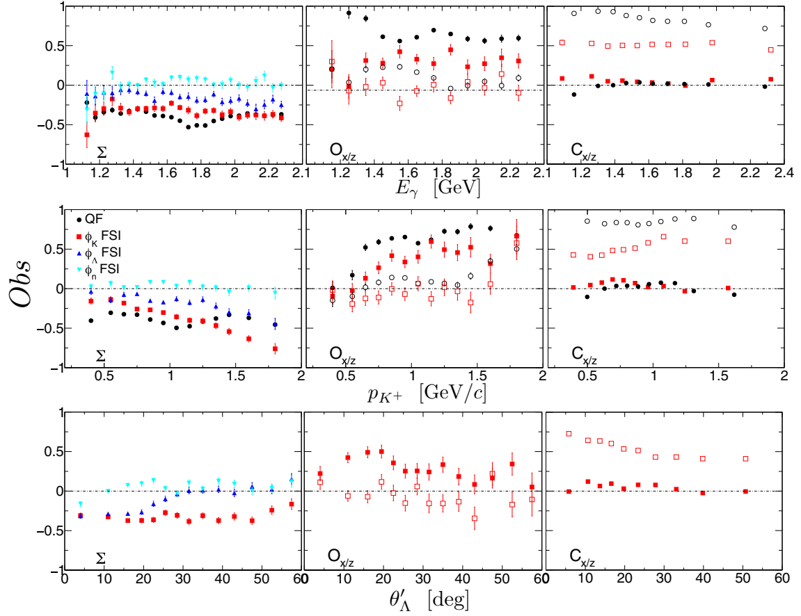
Fig. 9 First preliminary results for the quasi-free ( black points ) and FSI in the reaction \gamma d \rightarrow K^+ \Lambda n . The FSI results are determined using the kaon azimuthal angle ( red markers ) for the double polarisation observables. The beam spin-asymmetry is also determined using the hyperon and reconstructed neutron azimuthal distribution ( blue and cyan markers , respectively). For the double polarisation observables the solid markers represent the transverse polarisation transfers and the open markers the longitudinal polarisation transfers. The rows show the onefold differential results for photon energy, kaon momentum, and hyperon angles, respectively (Colour figure online)
