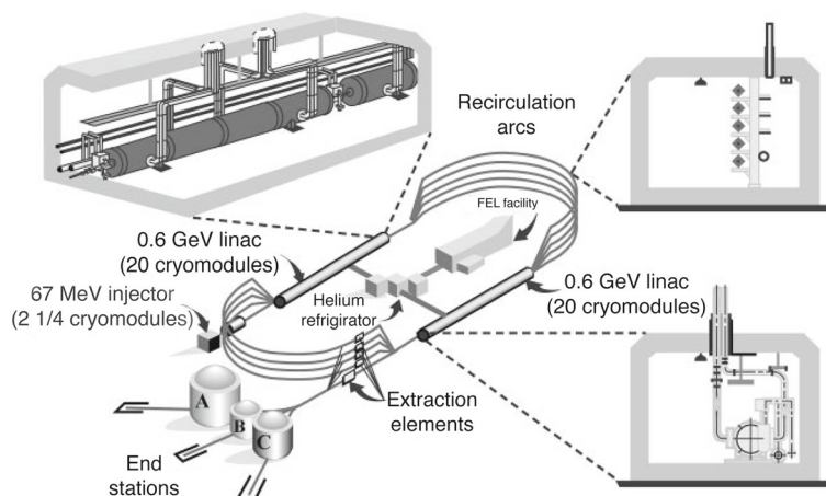
Fig. 1 Schematic CEBAF accelerator overview
