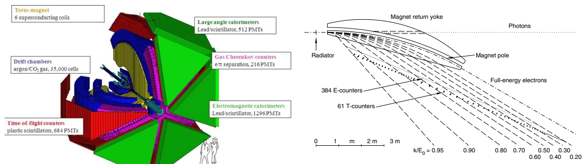
Fig. 2 Left Schematic CLAS detector. The kidney-shaped superconducting coils are shown in yellow, drift chambers in blue, Cerenkov counters in magenta, time-of-flight scintillators in red, and electromagnetic calorimeters in green. Right Hall B photon tagging system located upstream of the CLAS detector (Colour figure online)
