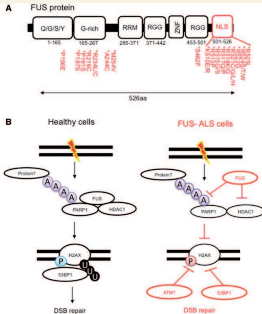
Figure 4 The familial ALS protein FUS promotes DNA repair. (A) A schematic depicting the structure of the FUS protein with ALS missense mutations highlighted. (B) FUS functions to regulate the DNA damage response through interactions with HDAC1 and PARP1. These interactions are important for H2AX phosphorylation (P) and 53BP1-mediated DSB repair. Loss of FUS or ALS-linked mutations leads to defective DSB repair and genomic instability.
