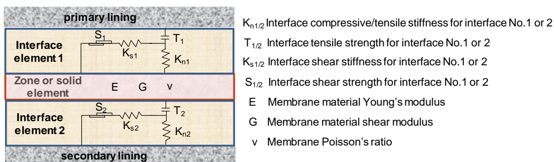
Figure 4. Membrane interface simulated using both zone or solid elements and interface elements (Option 3)
