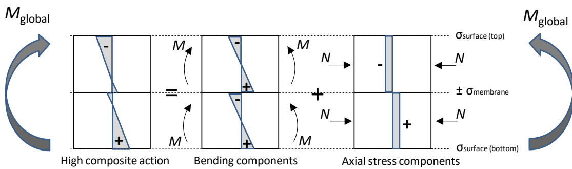
Figure 7 Breakdown of composite lining stresses due to global bending into bending and axial stress components
