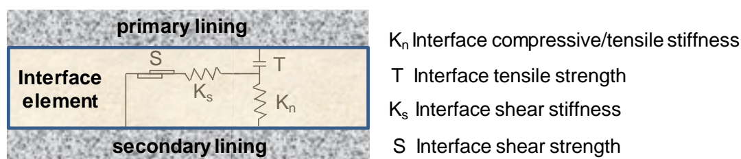
Figure 2. Membrane interface simulated using interface element (Option 1)
