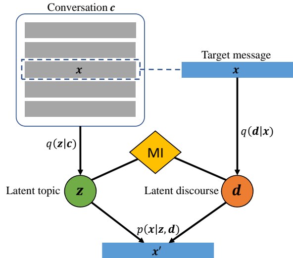
Figure 2: The architecture of our neural framework that jointly models latent topics and latent discourse.
