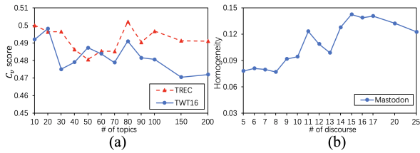
Figure 4: (a) The impact of topic numbers. The horizontal axis: the number of topics; The vertical axis: the C_v topic coherence. (b) The impact of discourse numbers. The horizontal axis: the number of discourse; The vertical axis: the homogeneity measure.
