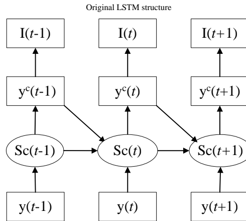
Fig. 2 LSTM network diagram.
