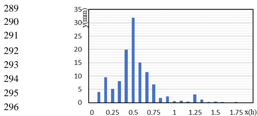
298 Fig.5. Two hours design rainstorm with the return period of 50 years
