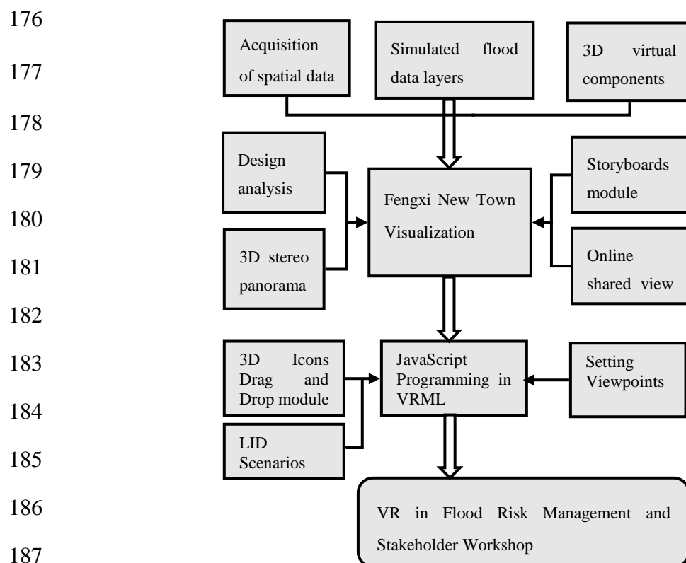
188 Fig.2. Framework for the development of the 3D model and simulation of design and actual flood in pilot 189 sponge city with LID scenarios. 190
