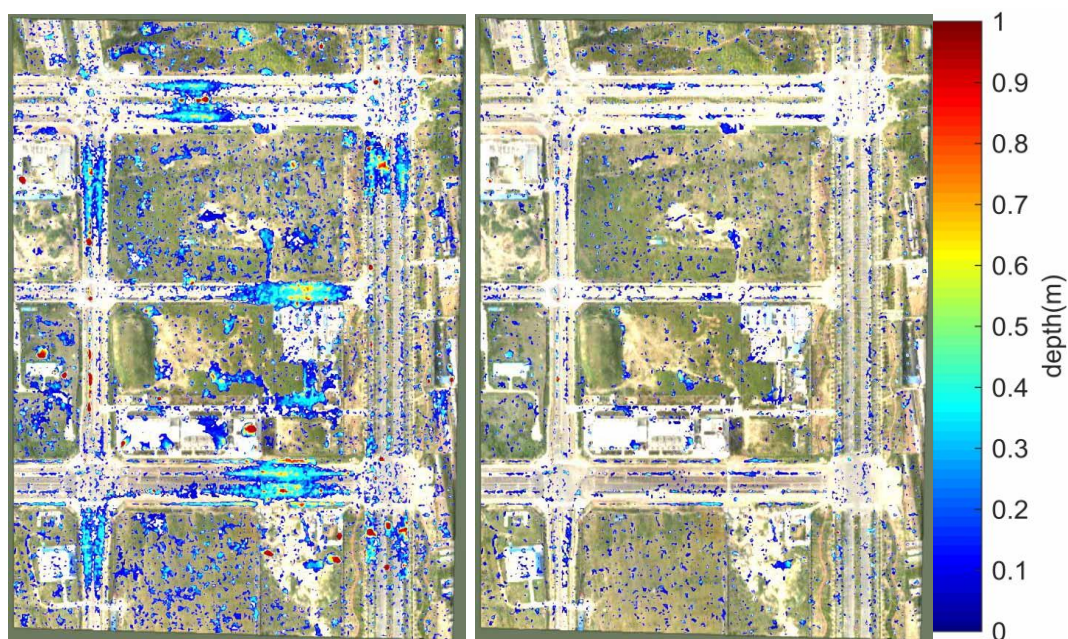
Fig.9. Flood inundation map with the return period of 50 years in Fengxi new town
