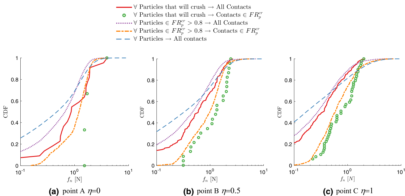
Fig. 11 CDF curves of the contact normal forces for different contacts subsets: all contacts on crushed particles; FR_p^{cr} contacts on crushed particles; all contacts; FR_p^{cr} contacts on all particles. For a given particle FR_p^{cr} is the maximum of F/F_{lim} , at its contacts
