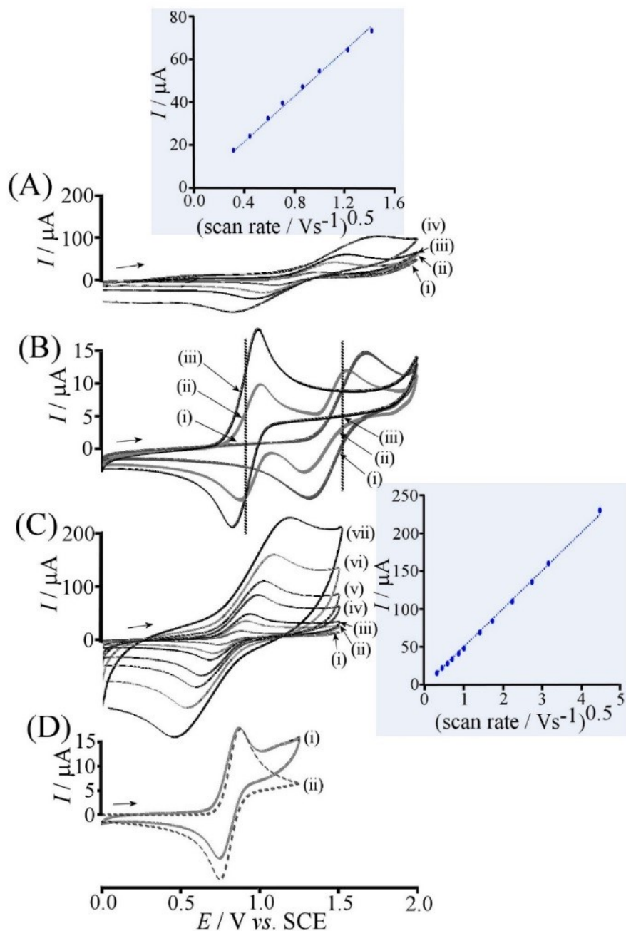
Figure 1. (A) Cyclic voltammogram (scan rate (i) 0.1 \text{V s}^{-1} , (ii) 0.5 \text{V s}^{-1} , (iii) 1 \text{V s}^{-1} , (iv) 3 \text{V s}^{-1} ) for 1 mM \text{Cl}_4\text{NHPI} in acetonitrile (0.05 M \text{NBu}_4\text{PF}_6 ). Inset: plot of I_p vs. (\text{scan rate})^{1/2} with a line of best fit. (B) Cyclic voltammograms (scan rate 0.1 \text{V s}^{-1} ) for the oxidation of 1 mM \text{Cl}_4\text{NHPI} in acetonitrile (0.05 M \text{NBu}_4\text{PF}_6 ) with added pyridine (with (i) 0, (ii) 0.1, (iii) 1 mM pyridine). (C) Cyclic voltammograms (scan rate (i) 0.1 \text{V s}^{-1} , (ii) 0.5 \text{V s}^{-1} , (iii) 1 \text{V s}^{-1} , (iv) 3 \text{V s}^{-1} , (v) 5 \text{V s}^{-1} , (vi) 10 \text{V s}^{-1} , (vii) 20 \text{V s}^{-1} ) for oxidation of 1 mM \text{Cl}_4\text{NHPI} in acetonitrile (0.05 M \text{NBu}_4\text{PF}_6 , 1 M pyridine). Inset: plot of I_p vs. (\text{scan rate})^{1/2} with a line of best fit. (D) Experimental (solid line) and simulated (hashed line) cyclic voltammogram (scan rate 0.1 \text{V s}^{-1} , 1.25 mM concentration, 1 M pyridine) for the oxidation of \text{Cl}_4\text{NHPI} .
