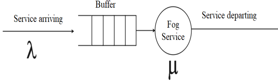
Figure 6: Queuing system
