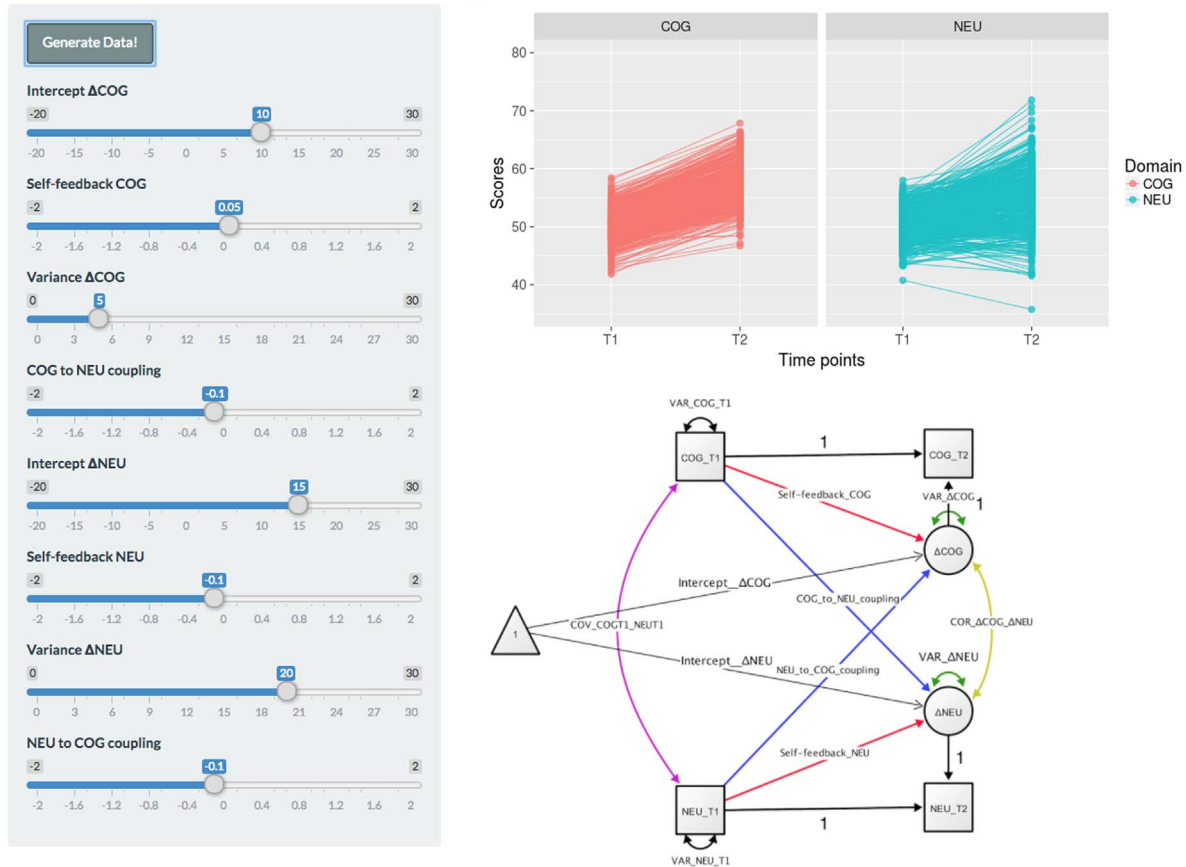
Fig. 7. Shiny interface. At the top users can select from three different latent change score models (Univariate, bivariate or dual). At the left, users can modify key parameters and select 'generate data' to simulate data with a given parametrisation. On the right, the raw data as well as the path model will be shown. This allows users to form an intuition of the effect of dynamic coupling. For instance, it can illustrate that even in the absence of significant changes within a domain, a coupling parameter from another domain can cause significant increases or decreases over time.
