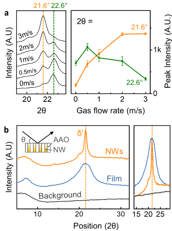
Figure 2. a) (left) XRD patterns of nanowire-filled templates crystallised at various assisted gas-flow rates. (right) Based on the normalised XRD patterns, the average intensity of the peak at 21.6^\circ and 22.6^\circ is plotted as a function of assisted-gas flow rate. b) XRD patterns of a nanowire-filled template (orange), melt-quenched film (blue), and silicon background (grey). The right image shows the magnification of the \delta' -phase range.
