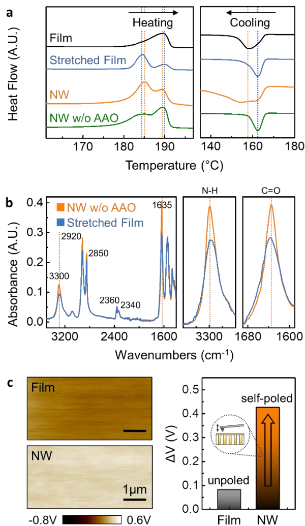
Figure 4. a) DSC thermograms for the melt-quenched film (black), additionally stretched film (blue), nanowires inside the template (orange), and template freed nanowires (green). b) FT-IR absorbance spectra for template-freed nanowires (orange) and additionally stretched film (blue). c) (left) KPFM potential images of the melt-quenched Nylon-11 film and the top surface of the self-poled nanowires filled template device. (right) The plot for the surface charge potential difference of each sample. The inset shows KPFM measured surface structure.
