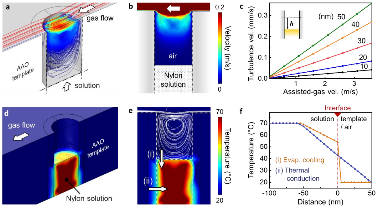
Figure 3. Numerical simulation results of turbulence flow generated by assisted gas-flow (3.1 m/s): a) 3D view and b) xz-plane view. c) Plot showing the relationship between the velocity of turbulent flow at different heights above the solution surface and assisted gas-flow rate. d) Simulation result of heat transfer around the solution-filled nano-pore. e) the xz-plane view of (d) with turbulent flow showing two dominant cooling mechanisms: (i) evaporative cooling and (ii) thermal conductive cooling. f) The temperature gradient from the centre of the solution to the air (orange) and template wall (blue). The initial temperature of the Nylon solution and assisted gas were taken to be 70\text{ }^{\circ}\text{C} and 20\text{ }^{\circ}\text{C} , respectively.
