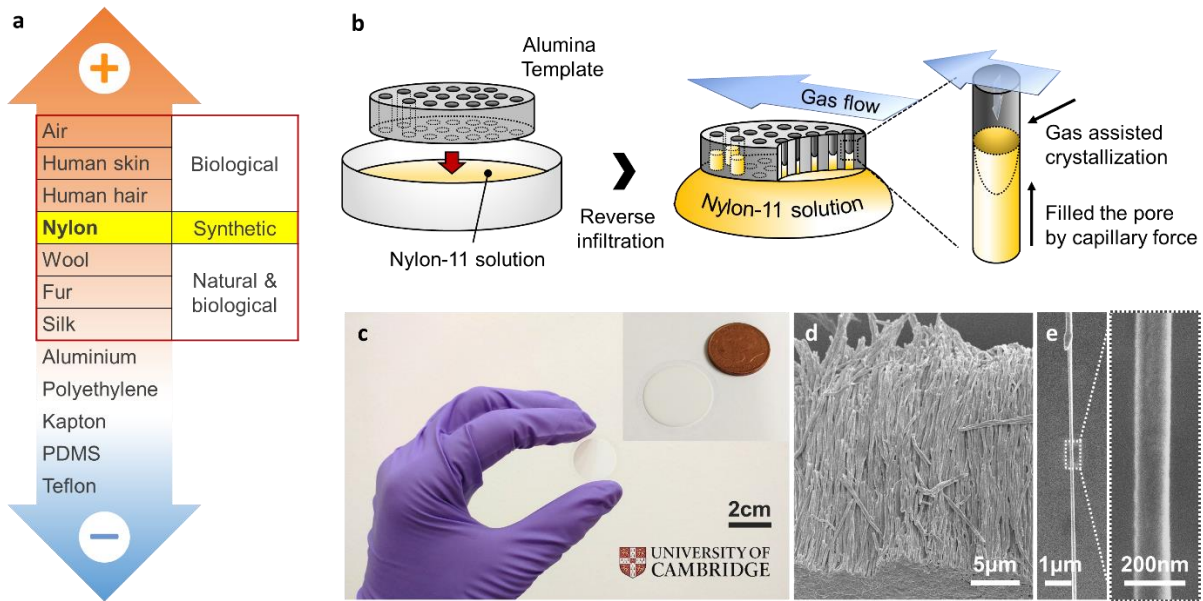
Figure 1. a) Triboelectric series of common materials with highlighted position of tribo-positive materials. b) Schematic of the nanowire fabrication procedure. c) Photographs of a fabricated nanowire-filled AAO template. The inset shows size comparison with a British one-pence coin. d, e) SEM images of template-freed nanowires and a single strand of Nylon nanowire, respectively.
