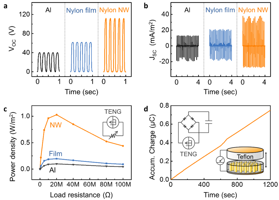
Figure 5. a) Open-circuit output voltages of triboelectric generators with different combinations of materials. The output voltage increases from \sim 40 V in the device with aluminium to \sim 110 V in the device with \delta' -phase Nylon nanowires. b) Short-circuit output current densities of the same triboelectric generators as in (a). c) The power density of different triboelectric devices as a function of variable load resistance. d) Charge accumulation of the nanowire-based TENG with respect to time. Left top and right bottom insets show the circuit structure and schematic of the TENG.
