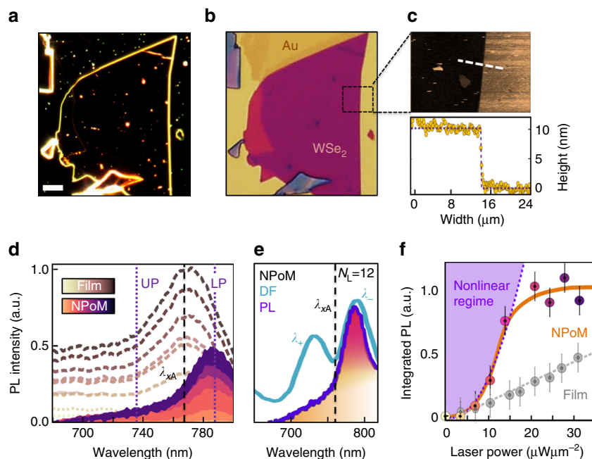
Fig. 2 WSe 2 stack properties. a Dark-field image with 10 \mu\text{m} scale bar (solid white line), b Bright-field and c AFM images of multilayer WSe 2 stack. The AFM height profile of flake edge (white dashed line) gives d = 10 \pm 0.4 nm, corresponding to 12 layers. d Power-dependent emission (Input power ranges from 0 to 30 \mu\text{W} \mu\text{m}^{-2} in steps of 2.5) at room temperature of the multilayer stack (brown) and NPoM (purple). Vertical lines mark A exciton absorption peak (black) and polariton peaks (purple). e Scattering and PL emission spectra on same NPoM, dashed line marks exciton absorption peak. f Scaling of integrated emission intensity with pump power for polaritons (orange curve) in NPoM (background subtracted) and (grey) excitons in multilayer on Au substrate. Error bars result from experimental noise and are extracted from the standard error of the background counts. Purple shading indicates the nonlinear emission regime
