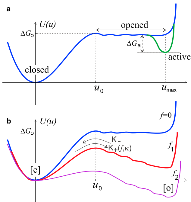
FIGURE 3 Shown here is a schematic of potential energy of different FAK conformations. (a) The force-free molecule has its native folded state [c] (compare with Fig. 2). The binding free energy \Delta G_o has to be overcome to separate the kinase from the FERM domain, after which there is a range of conformations of where roughly the same energy is achieved by further separating these two domains in the open state [o]. At full separation (distance u_{\max} ) the Src binding and kinase phosphorylation lead to the active state [a] of the protein, with the free energy gain \Delta G_a . (b) When a pulling force is applied to this system ( f_2 > f_1 > 0 ), the potential energy profile distorts, so that both [o] and [a] states shift down in energy by the same amount of -f \times u_{\max} . To see this figure in color, go online.
