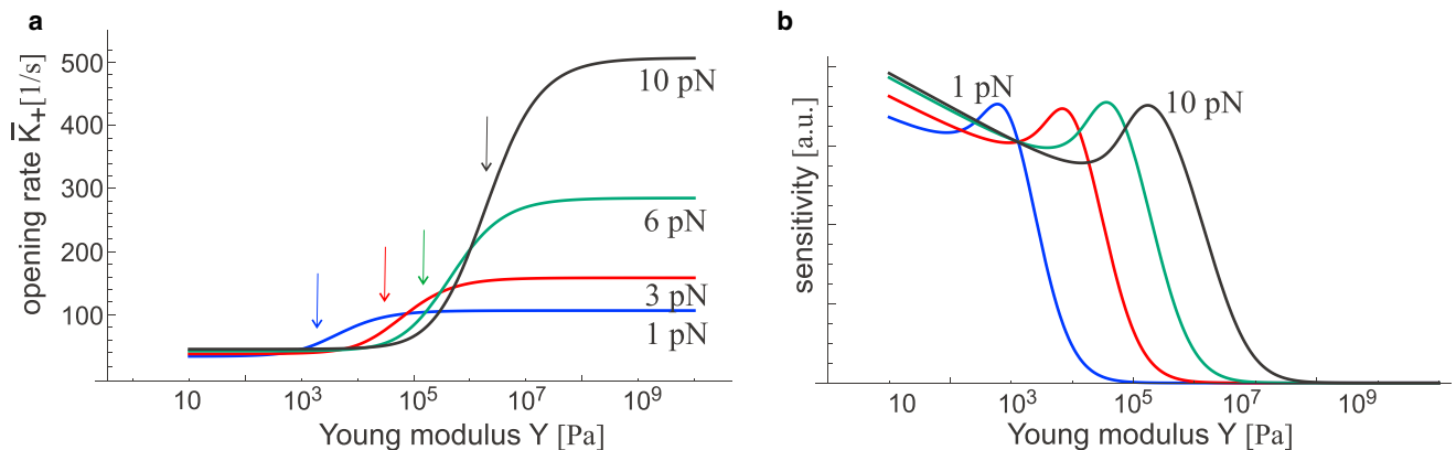
FIGURE 6 (a) The rate constant of the [c] \rightarrow [o] transition K_+(f, \kappa) is plotted against the substrate stiffness (on logarithmic scale) for several values of pulling force f . The arrows point at the inflection point on each curve, i.e., the region of maximum sensitivity. (b) Given here is the plot of sensitivity dK_+/dY for the same parameters, illustrating the maximum sensitivity range at each level of pulling force. To see this figure in color, go online.
