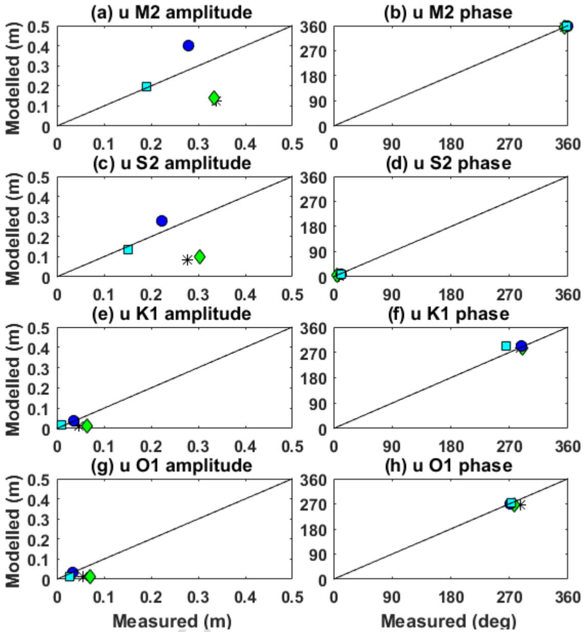
Figure 5: Comparison of the measured and predicted u velocity amplitudes and phases at the four ADCP sites for the: (a) M_2 amplitude; (b) M_2 phase; (c) S_2 amplitude; (d) S_2 phase; (e) K_1 amplitude; (f) K_1 phase; (g) O_1 amplitude; and (h) O_1 phase.
