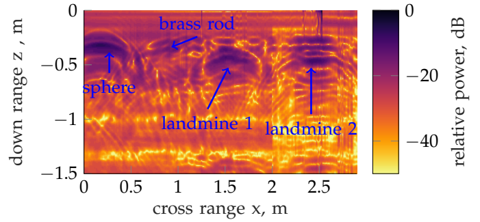
Figure 2: VV polarisation B-scan image of the radar scene with targets indicated.
