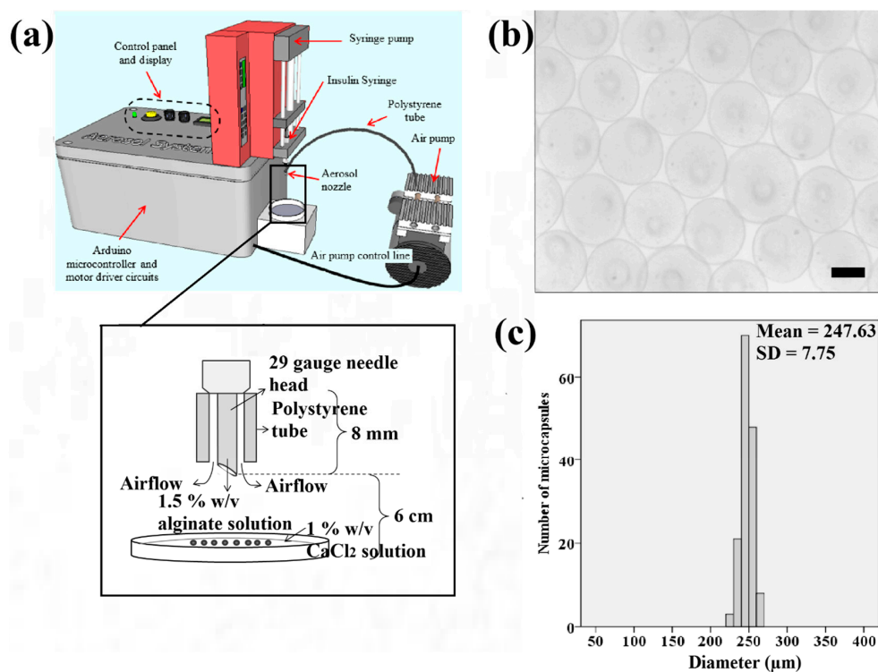
Figure 1. (a) Schematic illustration of the electronic aerosol microencapsulation system; (b) The photomicrographs of microcapsules (50× magnification) produced at the extrusion rate of 20 μL/min and air flow rate of 0.3 L/min (Scale bar: 200 μm); (c) Size distribution of the microcapsules.
