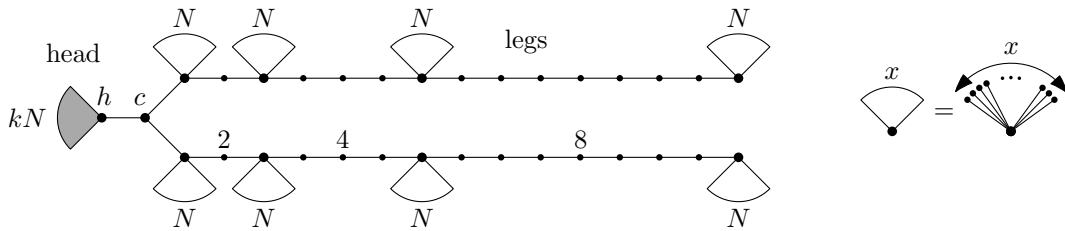
Figure 1: Player \mathbf{B} can ensure to get 2/3 - 1/k in t = 2 moves. A circular sector represents a large number x of leaves incident to one vertex (a “broom”). In the example, each leg has k = 4 brooms.
