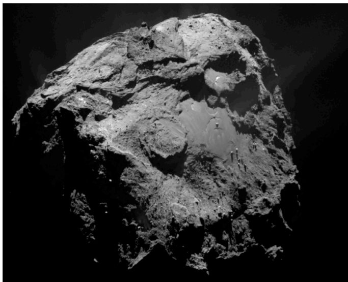
Fig. 16. The Bes and Imhotep sub-region definition. Left: OSIRIS image NAC_2015-08-01T23.55.10. Right: The 3D shape model. Bes mostly covers one long, thin face of the body of the nucleus with different topographical layers delineated by steep cliffs.
