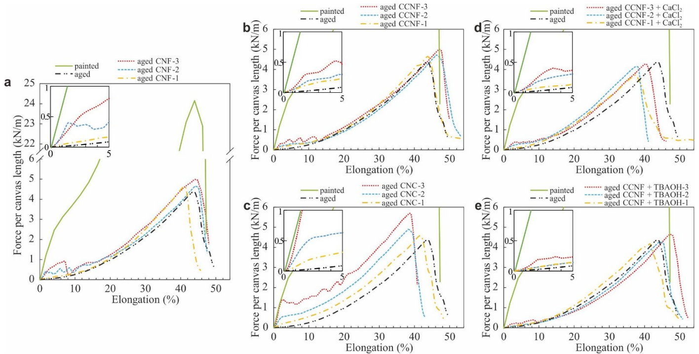
Fig. 4. Mechanical properties of the aged canvases coated with different number of coatings of: (a) CNF, (b) CCNF, (c) CNC, (d) CCNF + CaCl 2 and (e) CCNF + TBAOH. The curves for painted new canvas are also shown.
