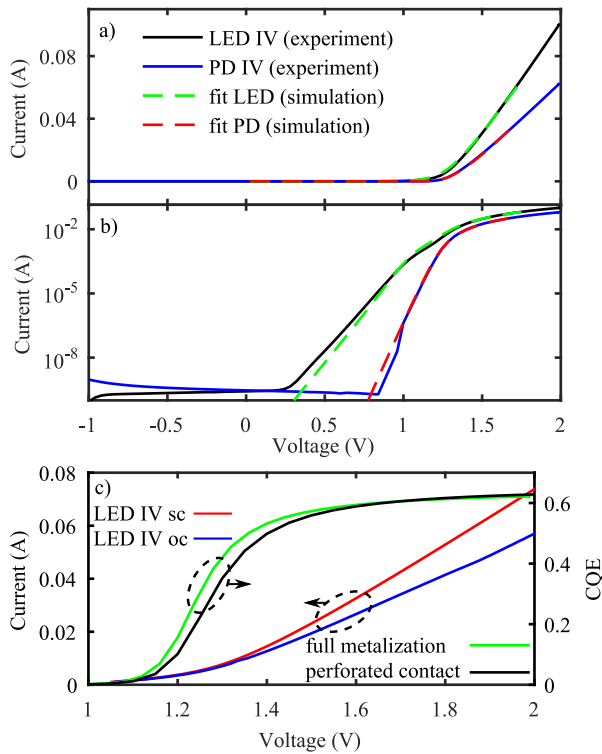
Figure 2. Typical experimentally measured I - V curves showing the current through the LED and PD as a function of voltage between the LED and common terminals for a DDS 245 with a 500 \mu\text{m} diameter and full metalization on a linear (a) and a semilogarithmic scale (b). The dashed lines show the corresponding results from the simulations. Experimental dependence of (left axis) the LED current on the voltage between the LED and common terminals when the PD of the 500 \mu\text{m} diameter DDS with perforated contact is open (oc) or short (sc) 250 circuited, and (right axis) the corresponding CQE for the same DDSs (c).
