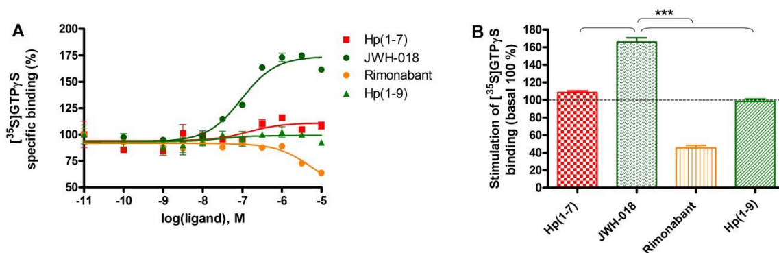
Figure 17. [ ^{35} S]GTP \gamma S binding stimulated by Hp(1-7), Hp(1-9) and cannabinoid ligands in rat brain membrane homogenate. JWH-018 and rimonabant were used as positive controls. Rat brain membranes were incubated with 0.05 nM [ ^{35} S]GTP \gamma S in the presence of increasing concentrations ( 10^{-10} - 10^{-5} M) of the indicated compounds. Non-specific binding was measured with 10 \mu M GTP \gamma S. Data are expressed as means \pm S.E.M., n = 3 . Statistical comparison of E_{max} and EC_{50} were performed by one-way ANOVA followed by the Bonferroni's multiple comparison test (***, P < 0.001 ).
