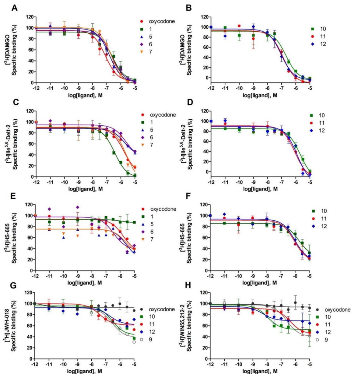
Figure 6. Concentration-dependent effects of the indicated compounds on equilibrium binding of [^3H]DAMGO (A-B, MOR), [^3H]Ile^{5,6}\text{-deltorphin-2} (C-D, DOR), [^3H]HS-665 (E-F, KOR), [^3H]JWH-018 and [^3H]WIN55,212-2 (G-H, CB receptors) in rat and guinea pig brain membrane homogenates. Figures represent the relative specific binding of the radioligands in the presence of increasing concentrations ( 10^{-11} – 10^{-5} M) of the synthetic compounds. Data are mean values \pm SEM ( n \geq 3 ). K_i values were calculated according to the Cheng–Prusoff equation ( K_i = EC_{50}/(1 + [ligand]/K_d) ) and are listed in Table 1.
