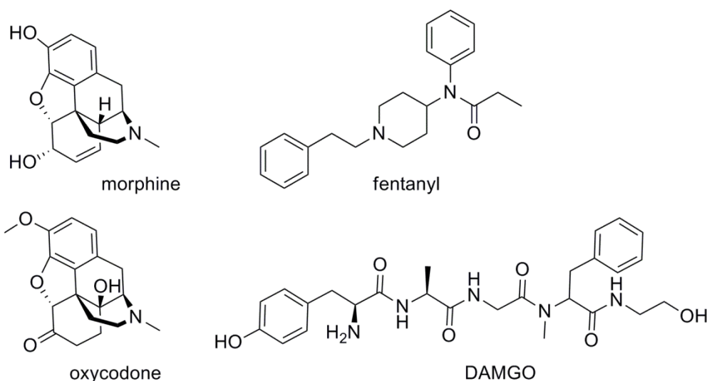
Figure 3. The structure of opioid receptor agonists.
