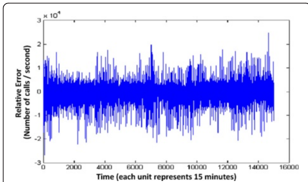
Figure 6 Relative error from training of previous half-year's data traffic load.
