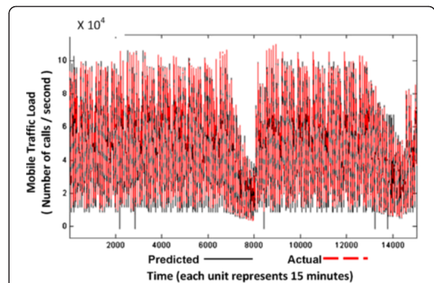
Figure 9 Prediction of the following half-year's data traffic rates based on the training of previous half-year's data traffic load.
