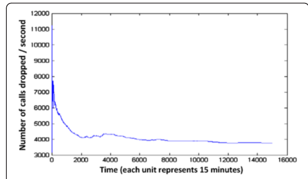
Figure 8 Rate of calls dropped from training of previous half-year's traffic load.
