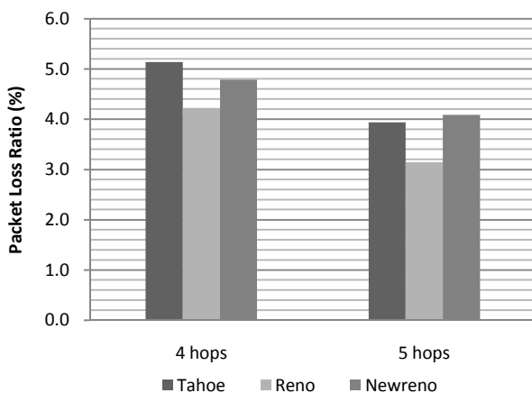
Fig. 10 Packet loss ratio for String topology
