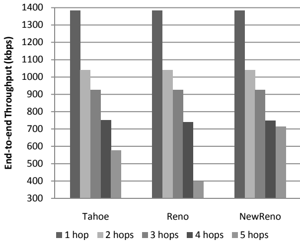
Fig. 6 Throughput for Grid topology
