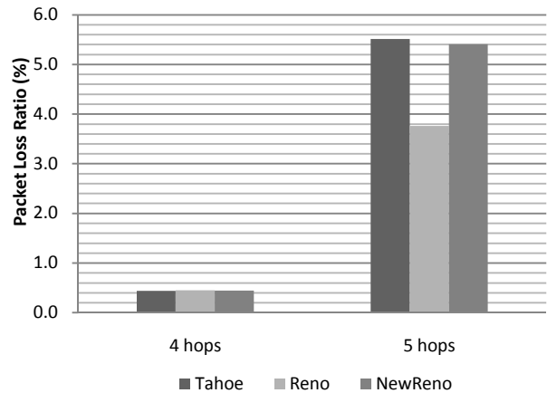
Fig. 12 Packet loss ratio for Grid topology
