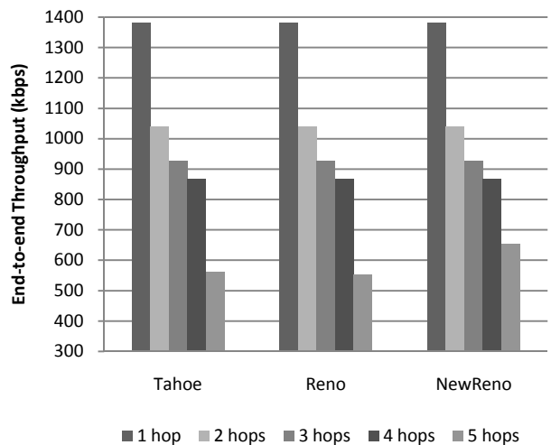
Fig. 5 Throughput for Ring topology
