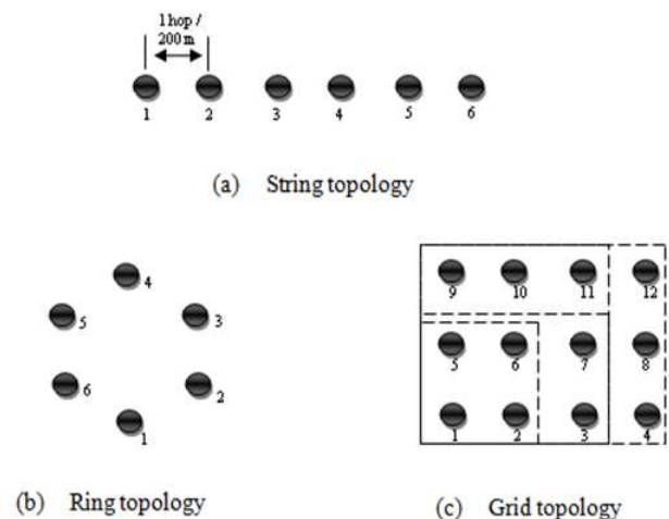
Fig. 3 Nodes configuration according to the different topologies- string, ring and grid
