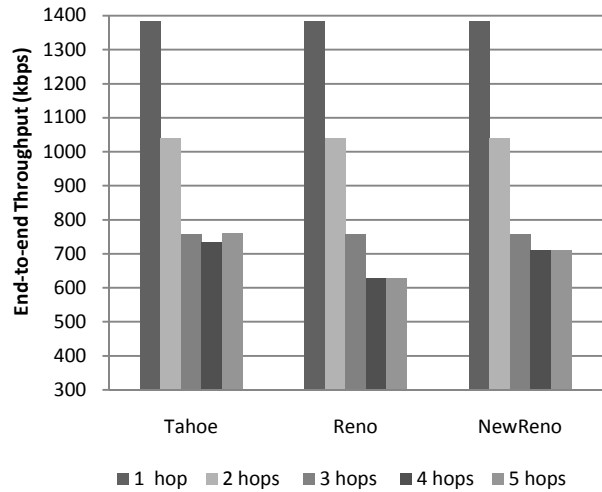
Fig. 4 Throughput for String topology
