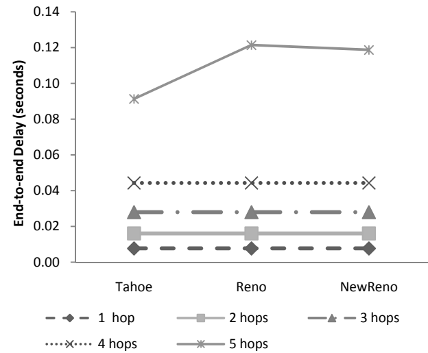
Fig. 8 End-to-end delay for Ring topology
