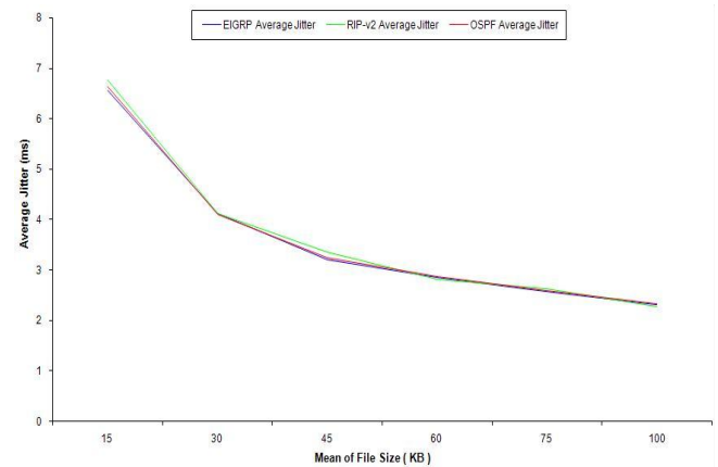
Fig. 10. Average Jitter Time in MD5 Secured Case
