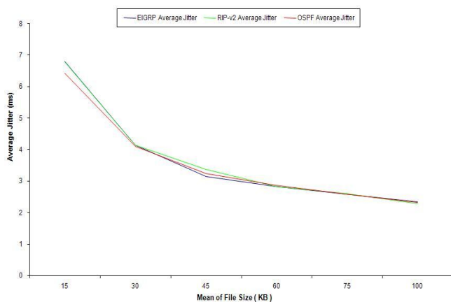
Fig. 9. Average Jitter Time in Non-secured Case
