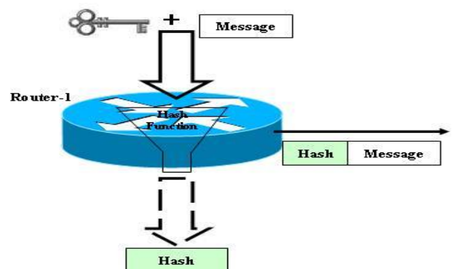
Figure 2. MD5 Neighbour Authentication at the Sending Router
