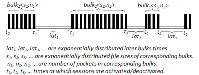
Figure 6. The Traffic Model
