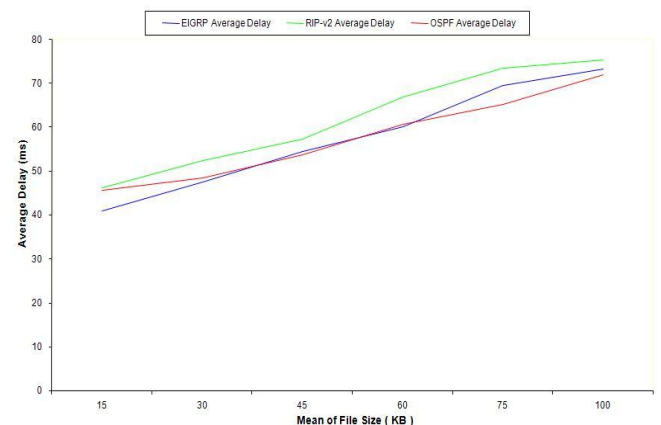
Fig. 7. Average Delay Time in Non-secured Case
