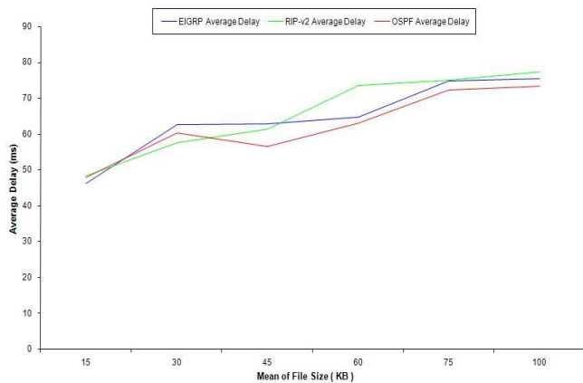
Fig. 8. Average Delay Time in MD5 Secured Case
